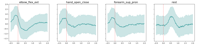
Figure 1: Grand-average cue-locked EEG waveforms after preprocessing (filtering and segmentation) for four behavioural classes.
