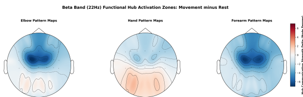
Figure 6 Trial-averaged connectivity-derived spatial patterns contrasting hand synergy epochs versus rest on the standard Graz layout. Activation is appropriately localized to the sensorimotor areas.
