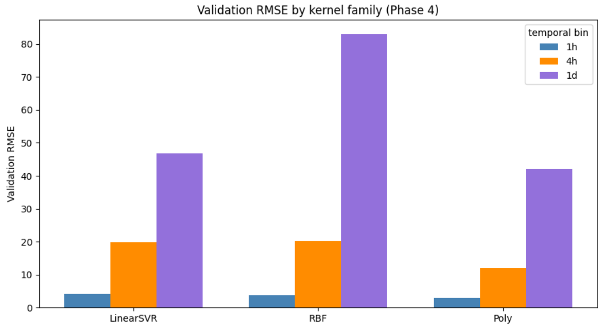
Figure 1: Validation RMSE by kernel family across all configurations.
