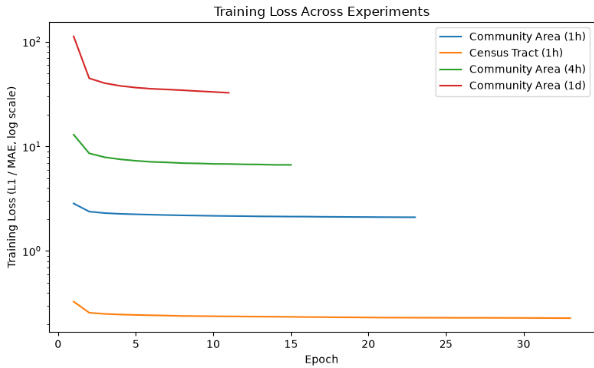
Figure 5: Training loss curves across all four experiments.
