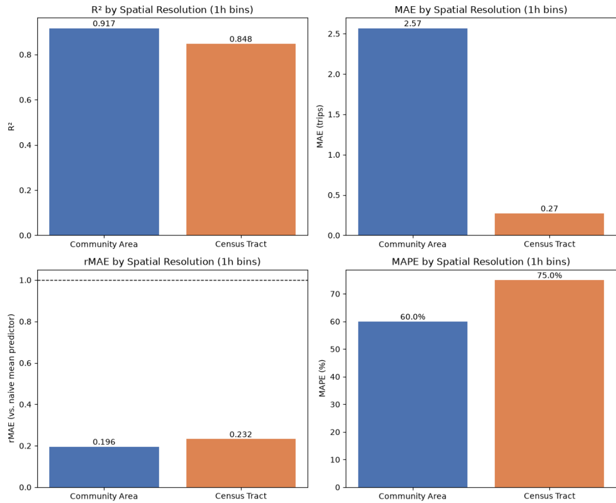
Figure 3: Neural network performance by spatial resolution (1h bins).
