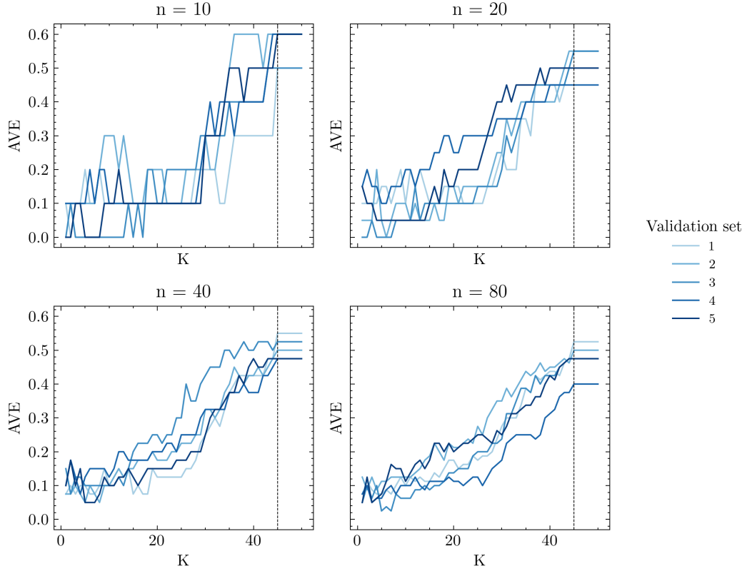
Figure 1: Average validation error for different sizes of validation sets
