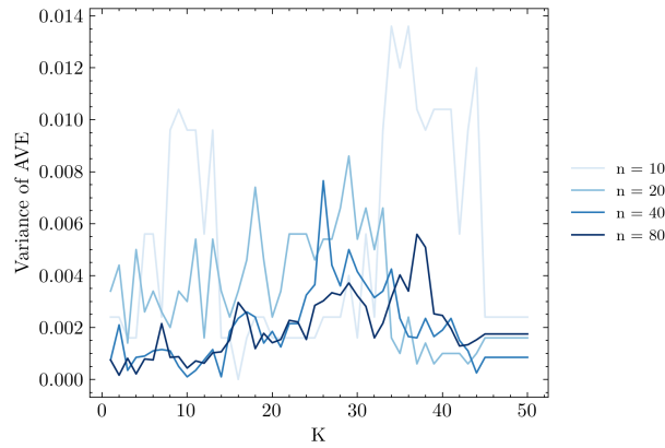
Figure 2: Variance of validation error
