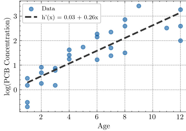
Figure 3: Visualizing the fitted model (2)
