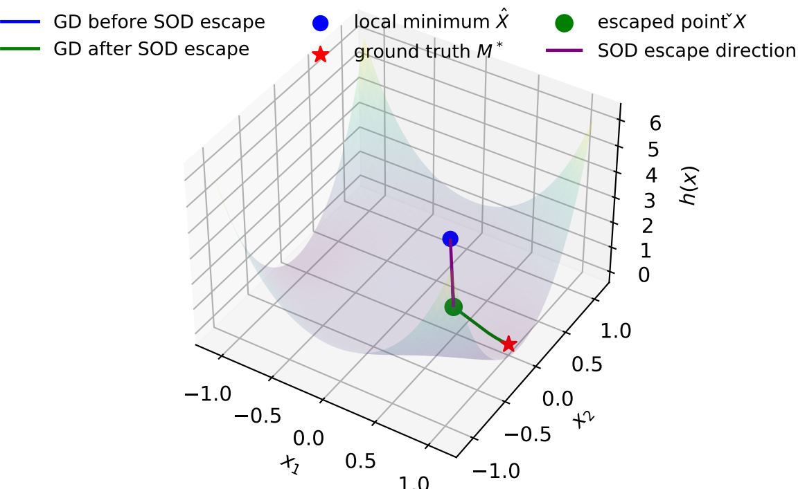
Surface + GD Trajectory (with SOD escape, eta is 0.001)
