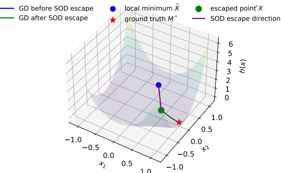
Surface + GD Trajectory (with SOD escape, eta is 0.01)
