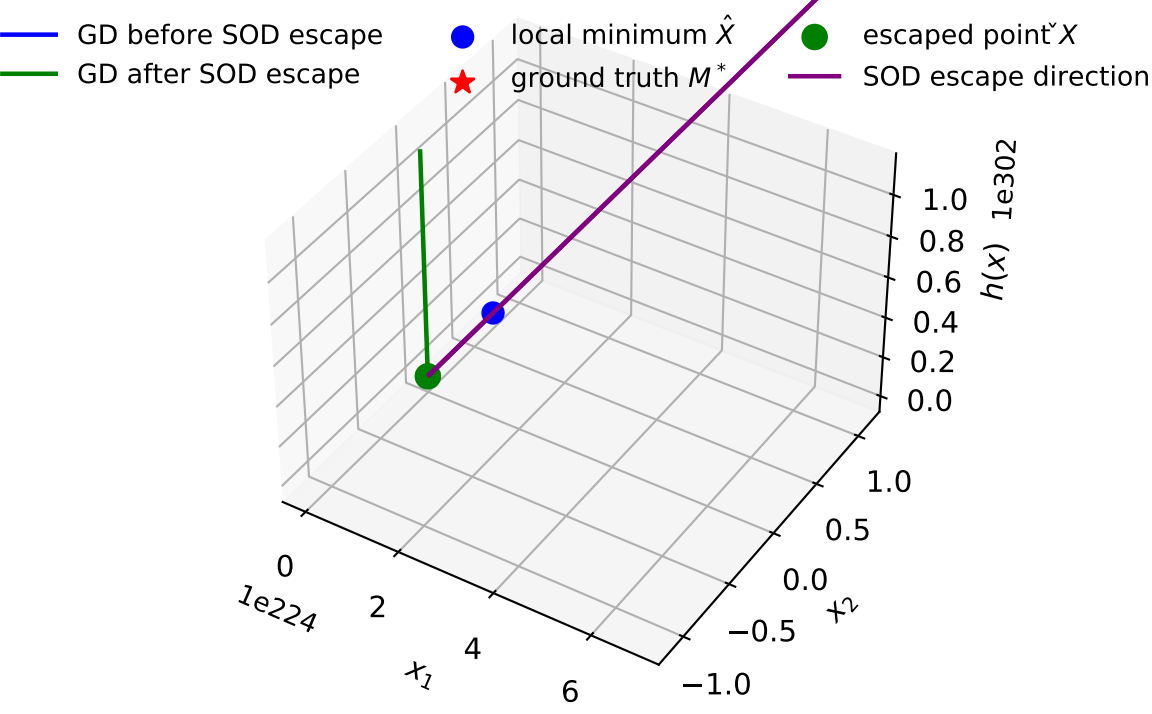
Surface + GD Trajectory (with SOD escape, eta is 0.1)
