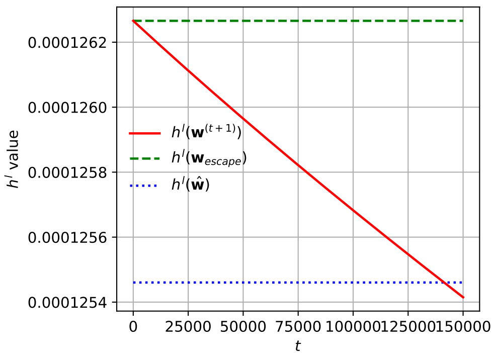
Lifted Loss vs t (eta=0.1)
