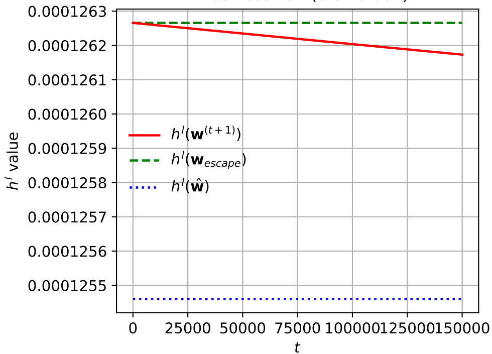
Lifted Loss vs t (eta=0.01)
