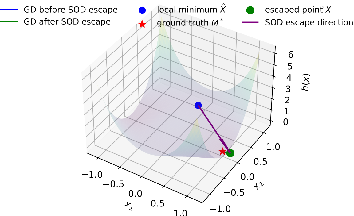
Surface + GD Trajectory (with SOD escape, l is 5)
