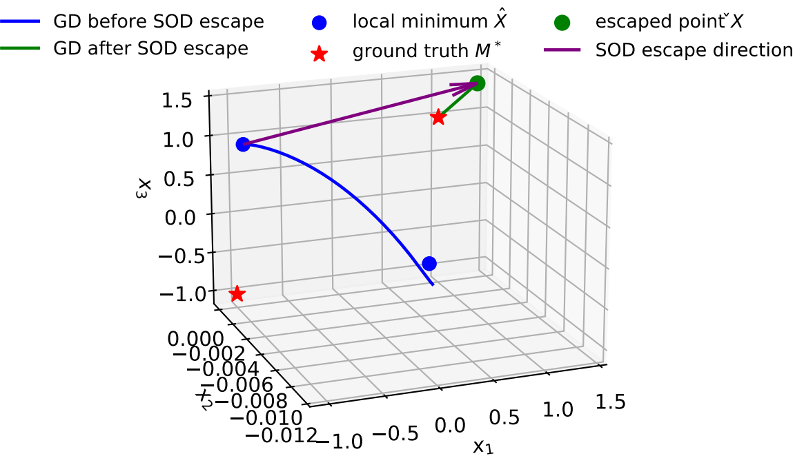
Trajectory in 3D Space (with SOD escape, l is 9)
