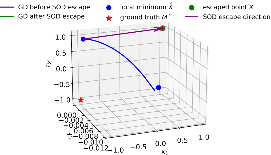
Trajectory in 3D Space (with SOD escape, l is 11)
