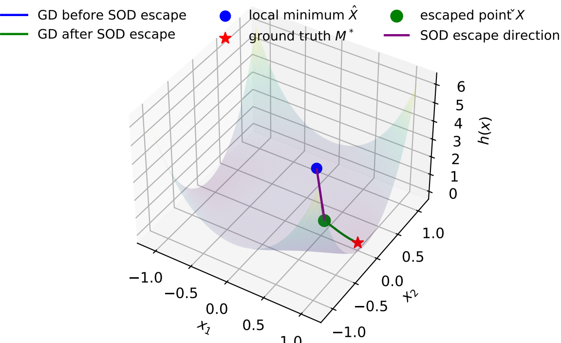
Surface + GD Trajectory (with SOD escape, rho is 0.1)
