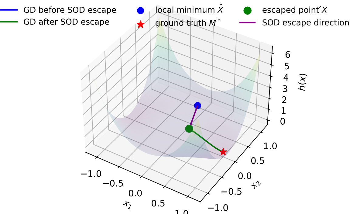
Surface + GD Trajectory (with SOD escape, rho is 0.01)
