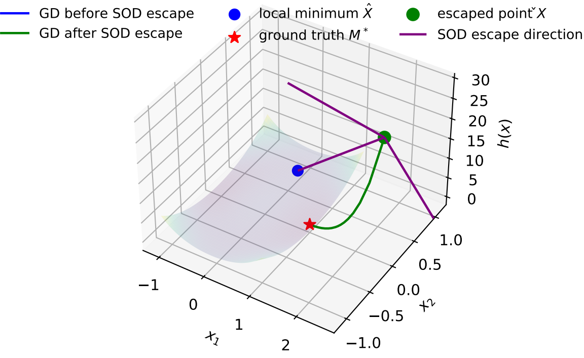
Surface + GD Trajectory (with SOD escape, rho is 1.0)
