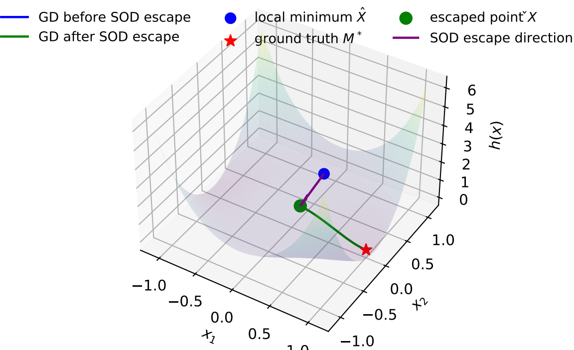
Surface + GD Trajectory (with SOD escape, rho is 0.001)
