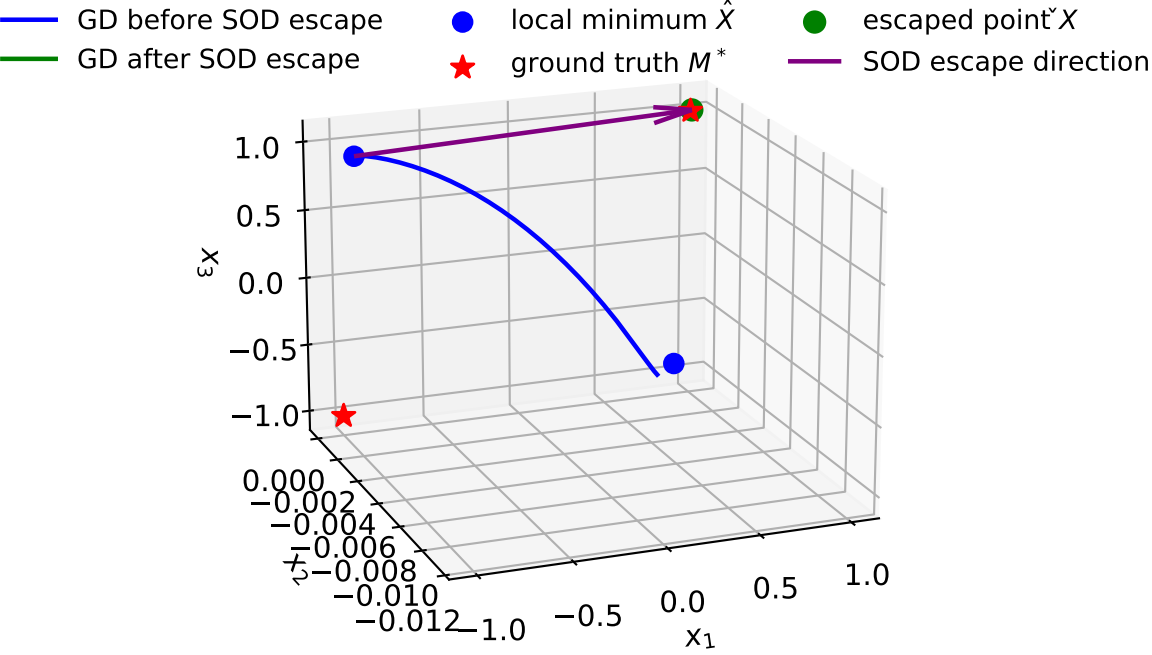
Trajectory in 3D Space (with SOD escape, rho is 3)
