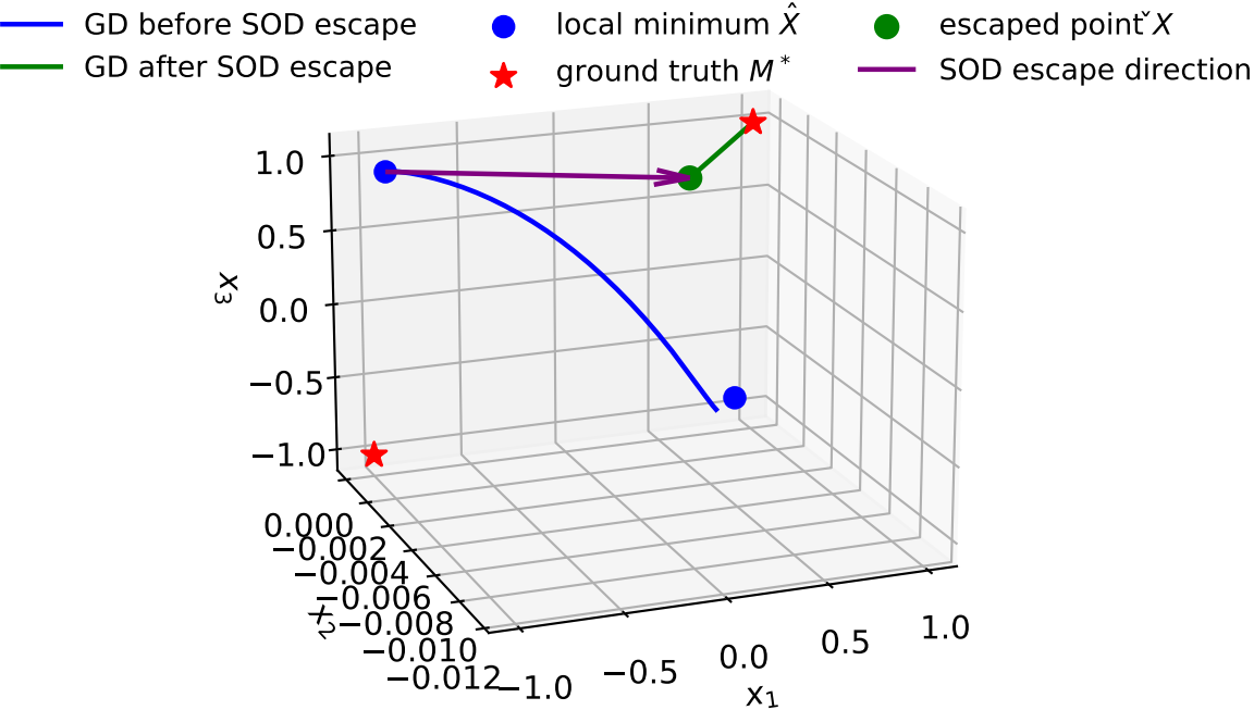
Trajectory in 3D Space (with SOD escape, rho is 0.03)
