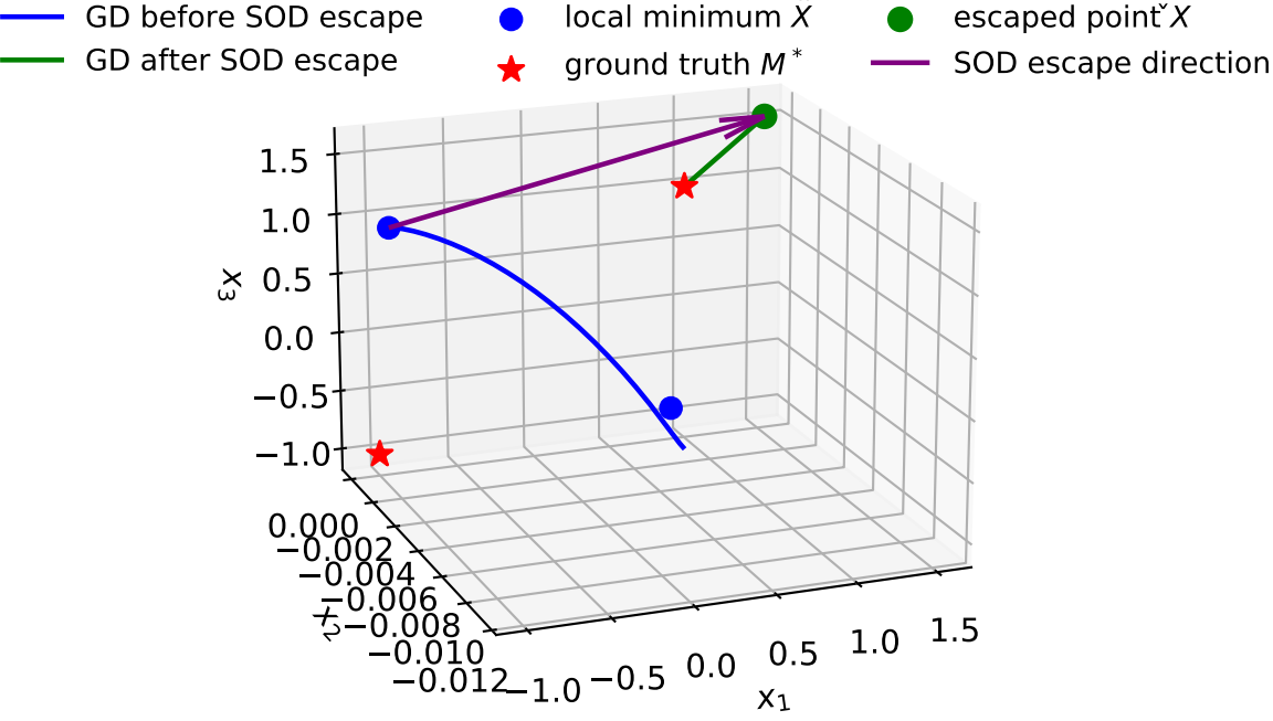
Trajectory in 3D Space (with SOD escape, rho is 30)
