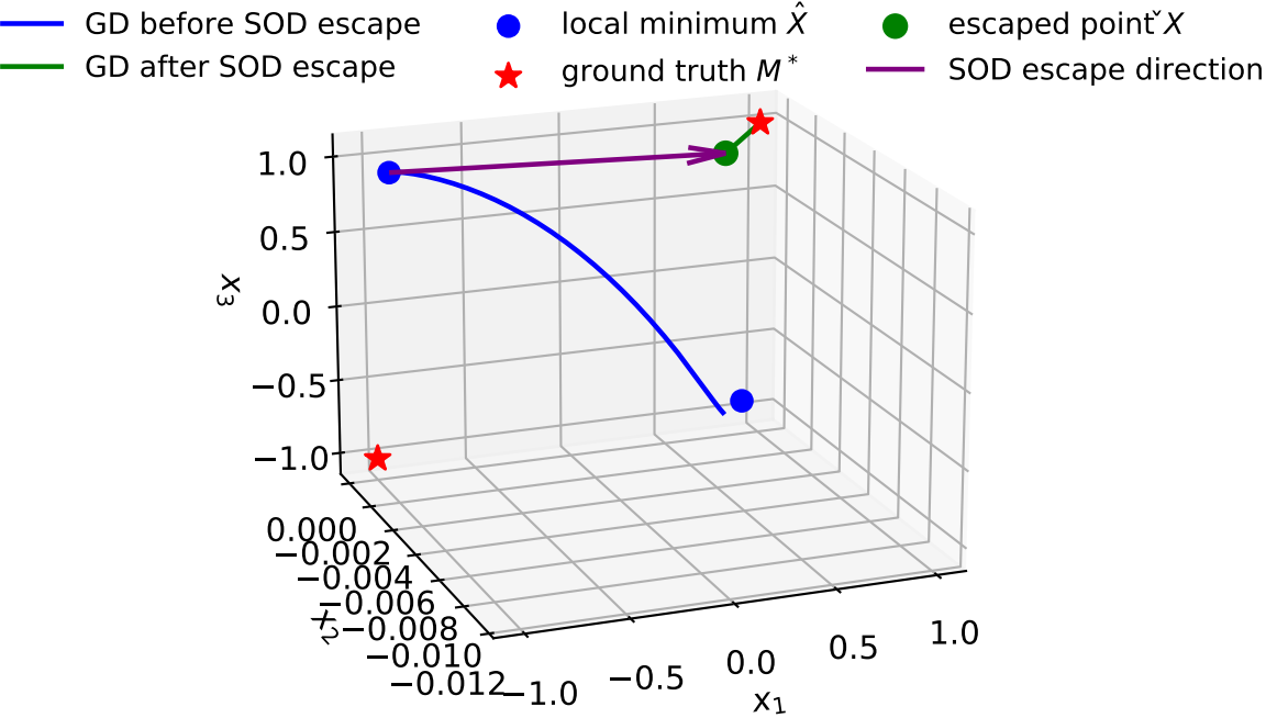
Trajectory in 3D Space (with SOD escape, rho is 0.3)
