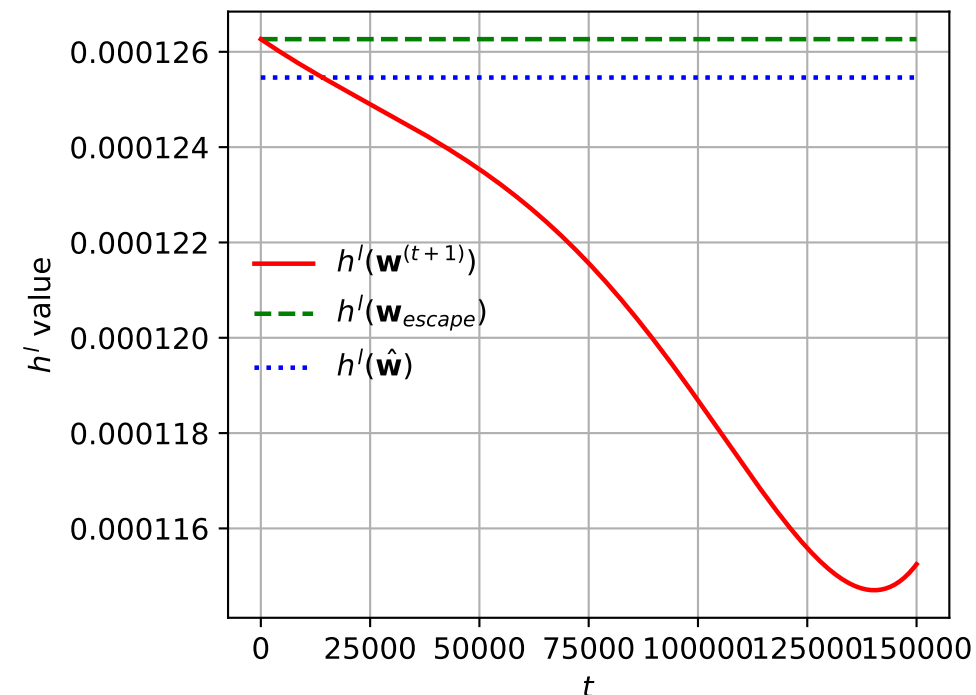
Lifted Loss vs t (rho=1.0)
