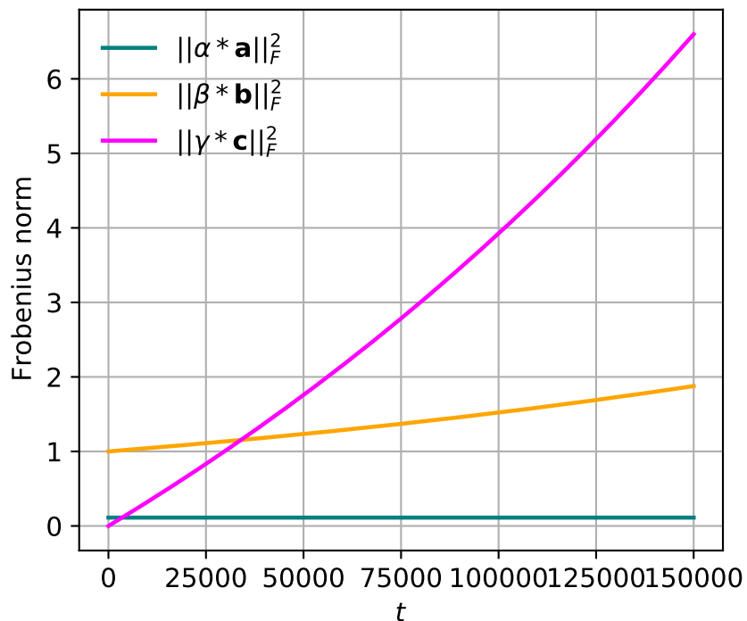
Norms vs t (rho=10.0)
