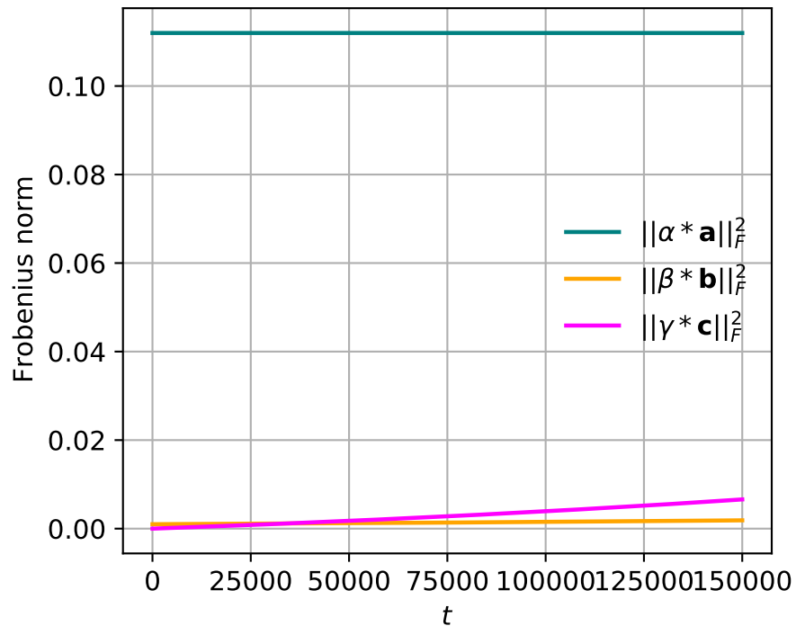
Norms vs t (rho=0.01)
