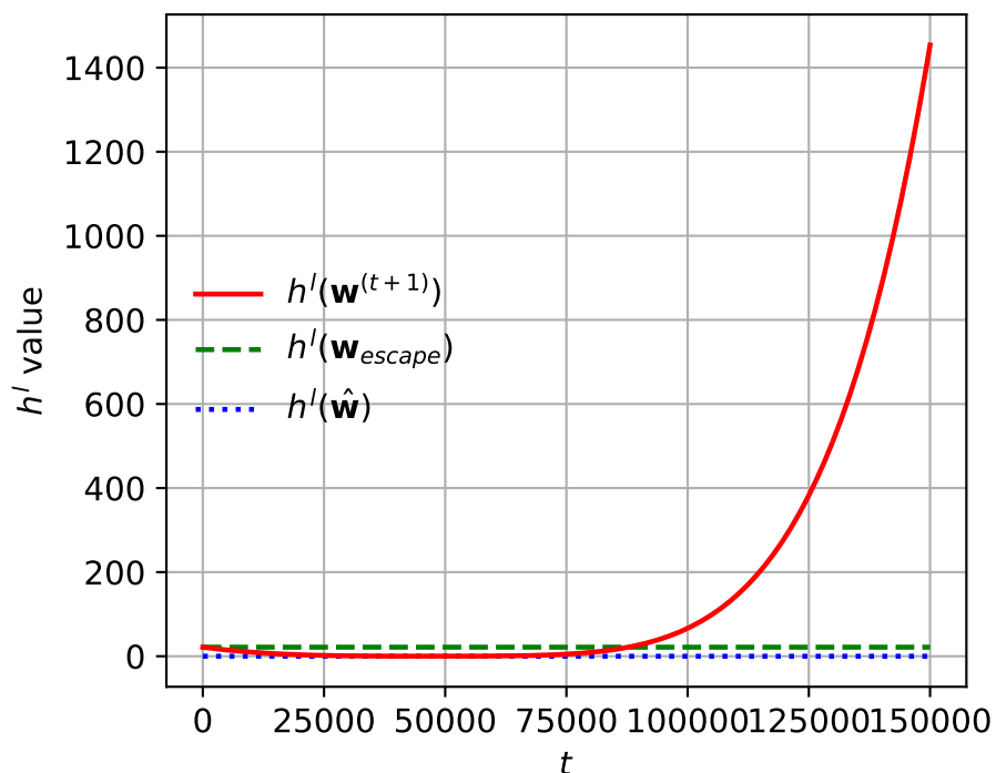
Lifted Loss vs t (rho=10.0)
