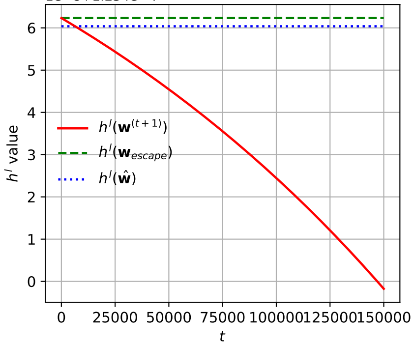
Lifted Loss vs t (rho=0.01)
