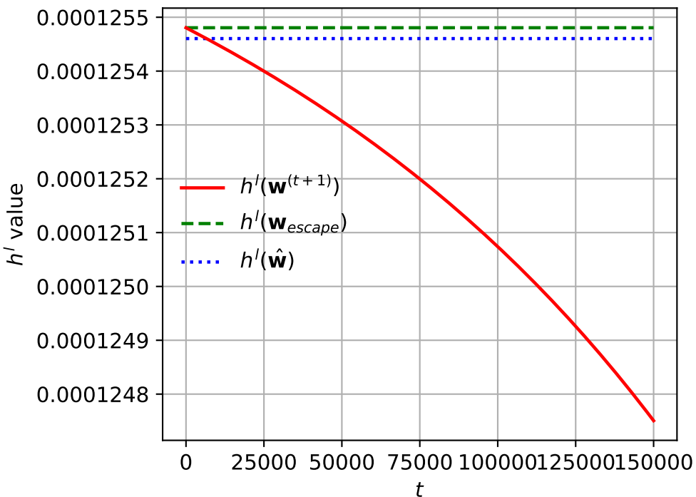
Lifted Loss vs t (rho=0.1)
