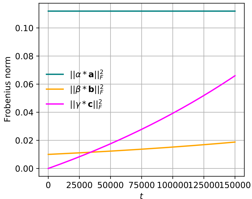
Norms vs t (rho=0.1)
