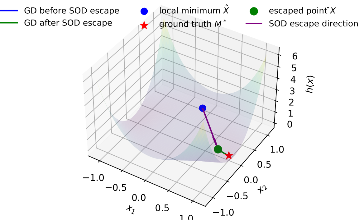
Surface + GD Trajectory (with SOD escape, t is 660)
