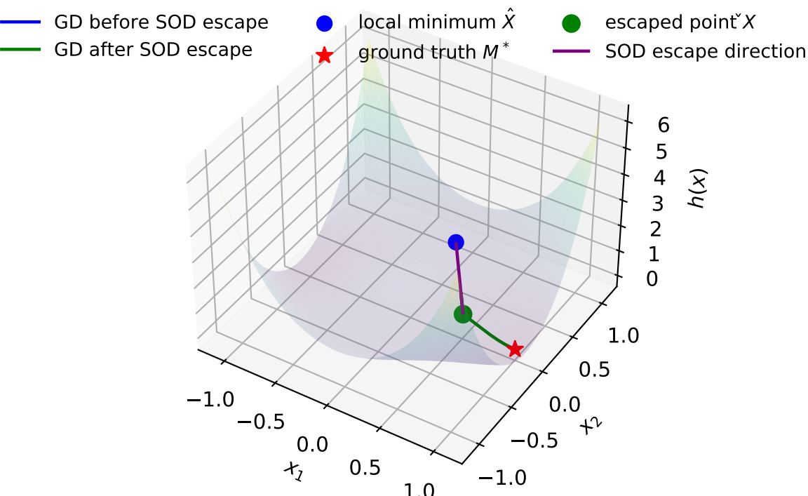
Surface + GD Trajectory (with SOD escape, t is 360)
