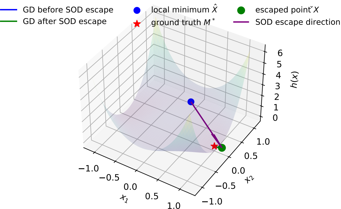
Surface + GD Trajectory (with SOD escape, t is 960)
