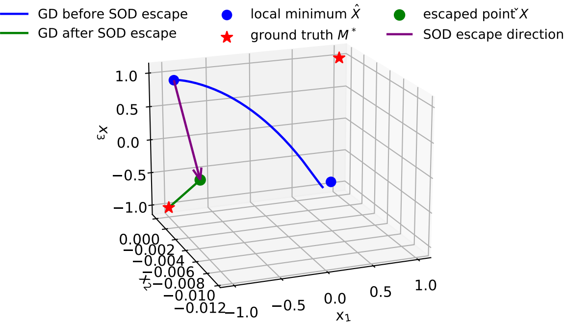
Trajectory in 3D Space (with SOD escape, t is 9000)
