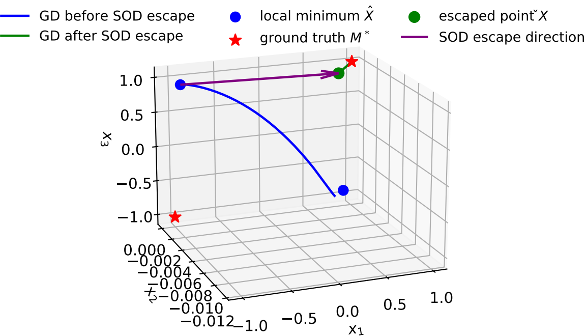
Trajectory in 3D Space (with SOD escape, t is 39000)
