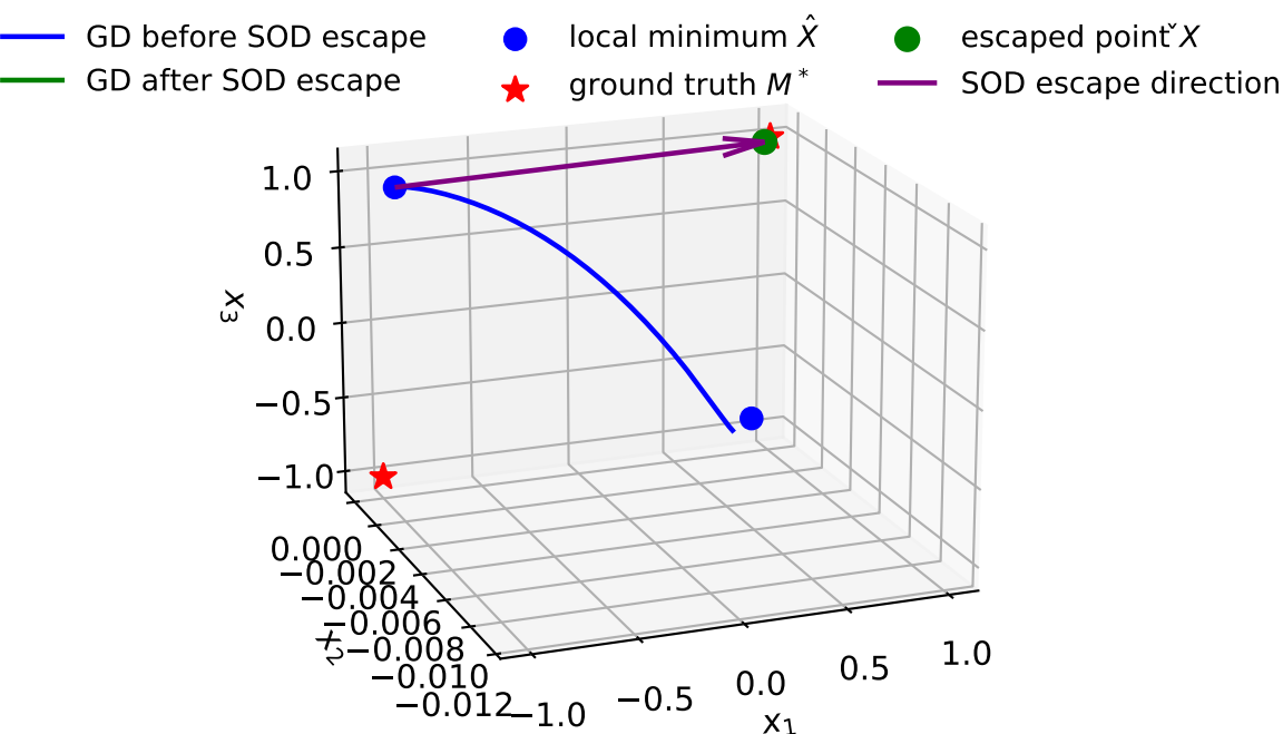
Trajectory in 3D Space (with SOD escape, t is 69000)
