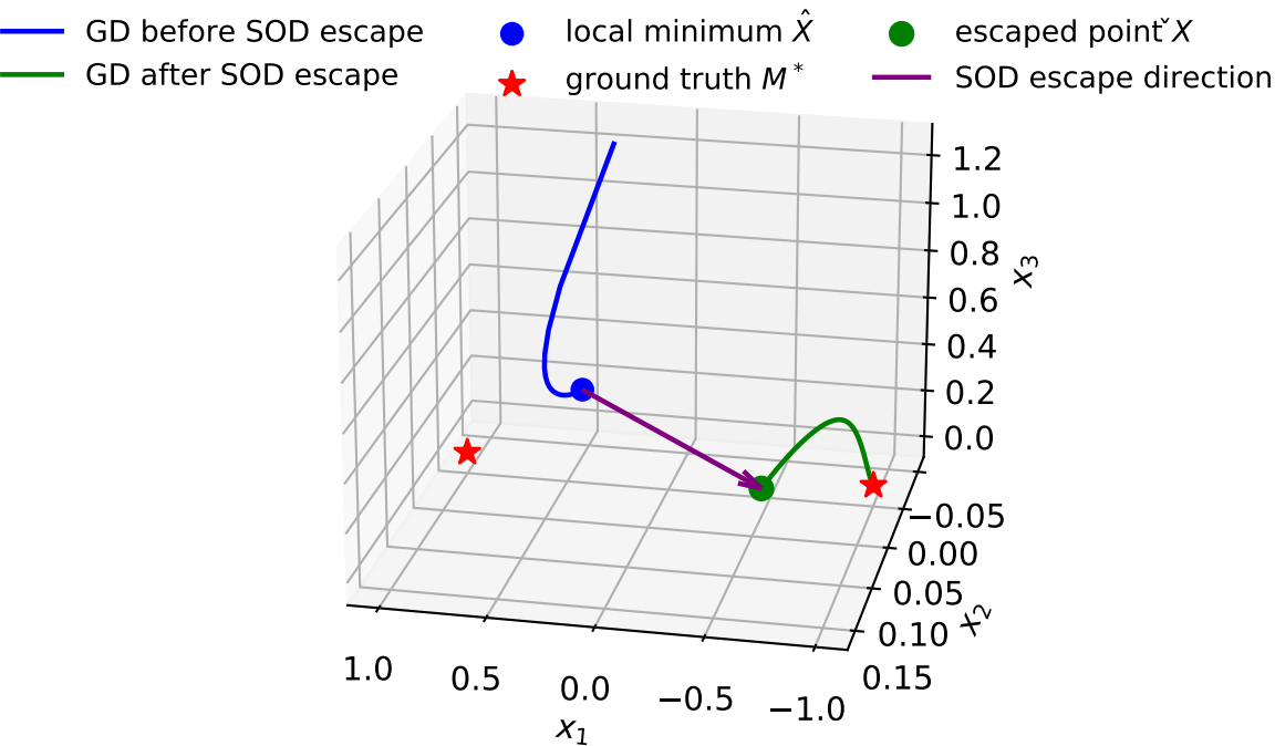
Trajectory in 3D Space (with SOD escape, t is 5000)
