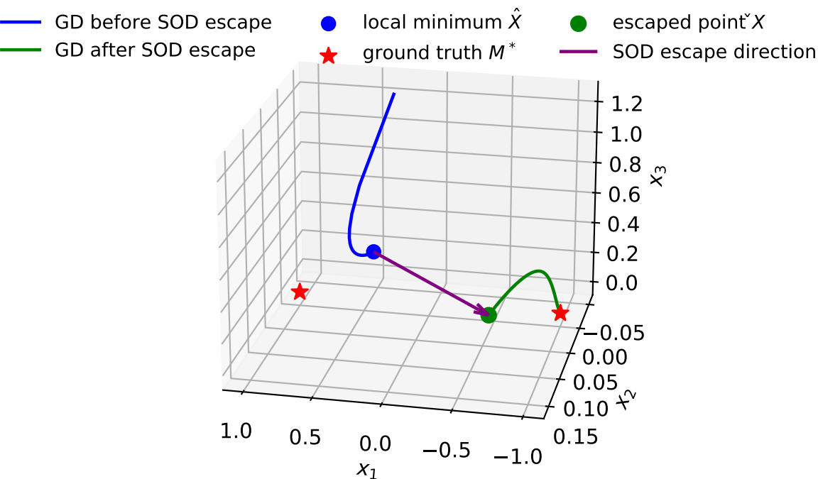
Trajectory in 3D Space (with SOD escape, t is 100000)
