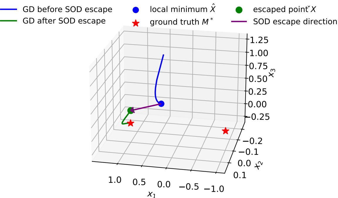
Trajectory in 3D Space (with SOD escape, t is 500000)
