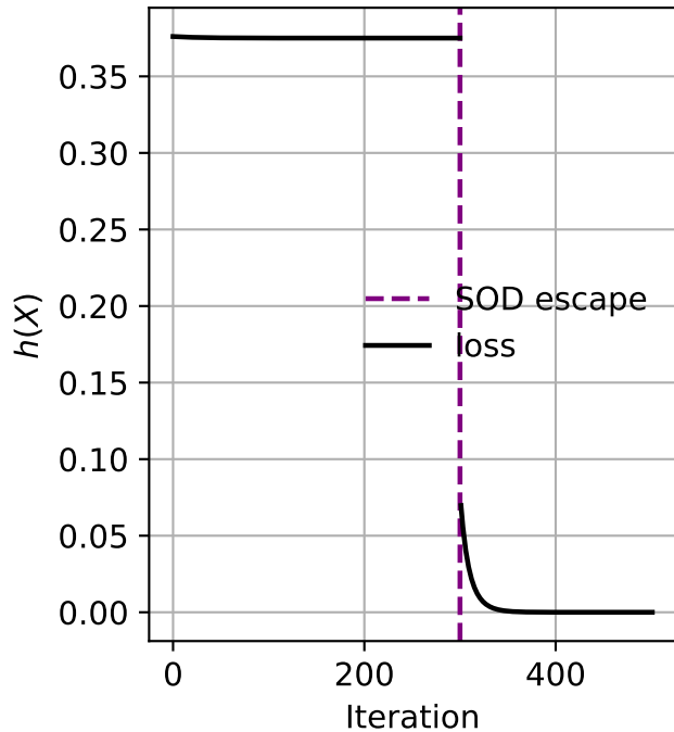
Loss vs Iteration
