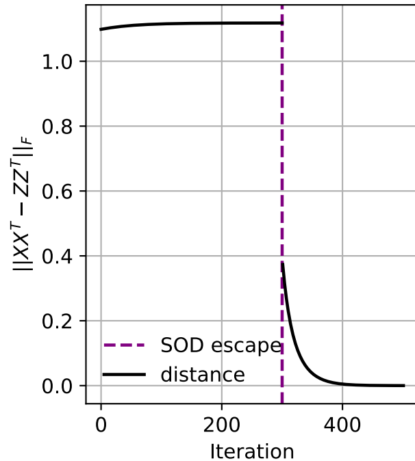
Distance vs Iteration
