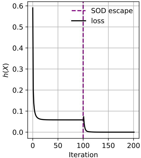
Loss vs Iteration
