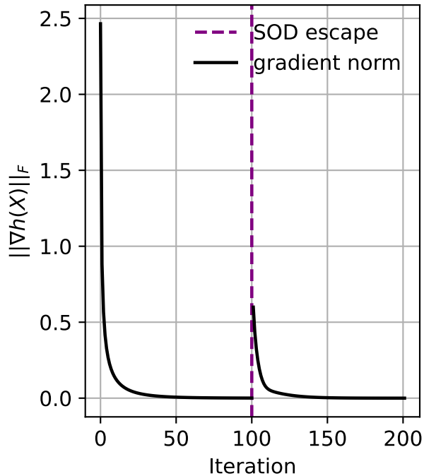
Gradient Norm vs Iteration
