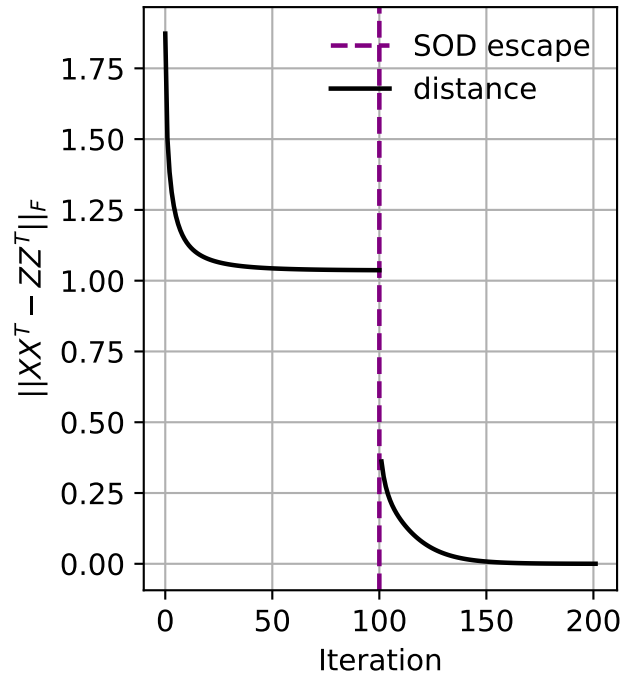
Distance vs Iteration
