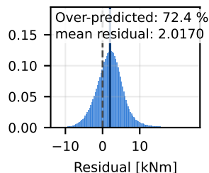
Roll RMS
