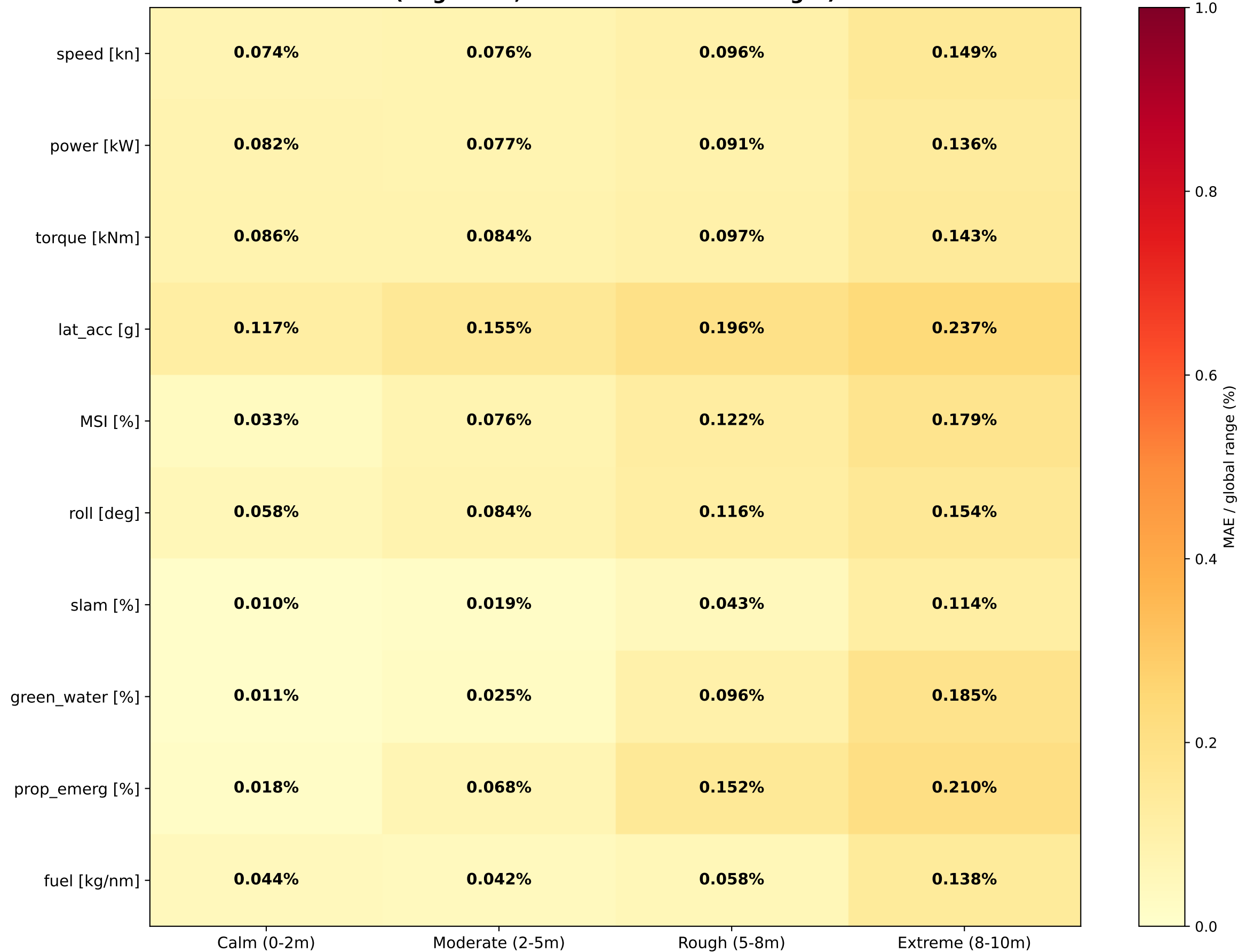
Relative Error (MAE / global output range, %) by Output and Sea Condition (Regressor, rows with a defined target)
