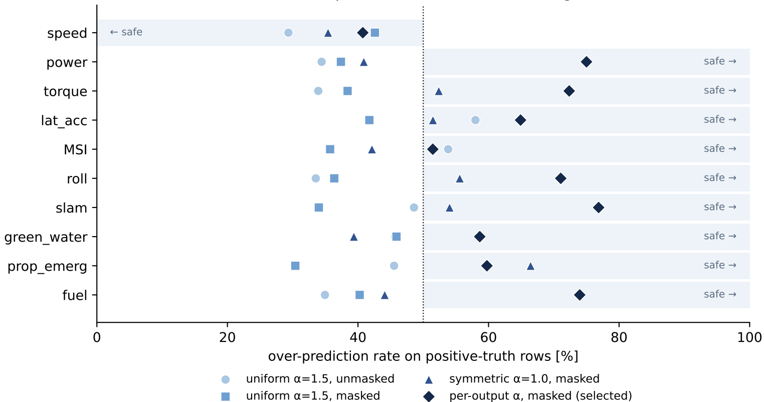
Which side does each output err on, per loss configuration (shaded half = the output's safe side; same training and test rows)
