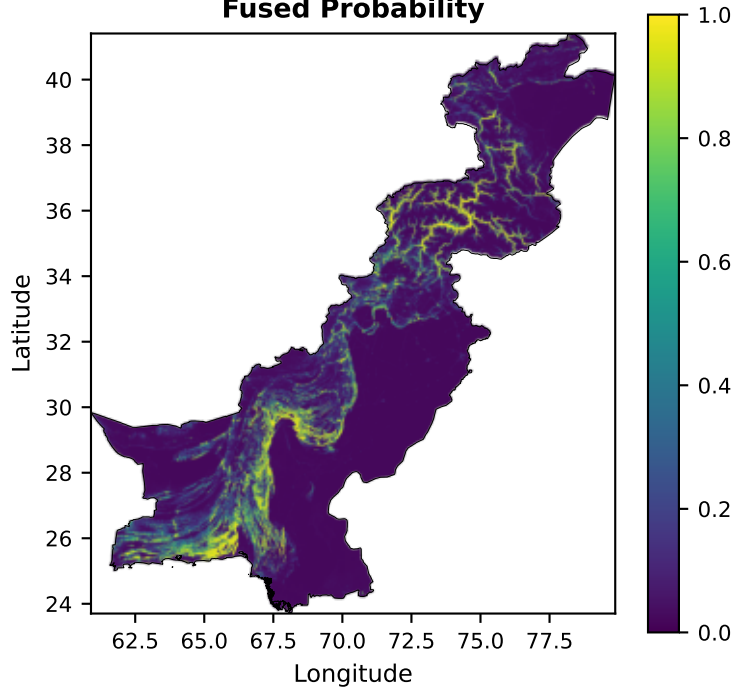
Fused Probability
