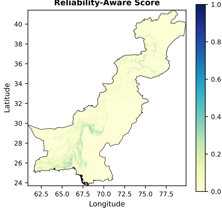
Reliability-Aware Score
