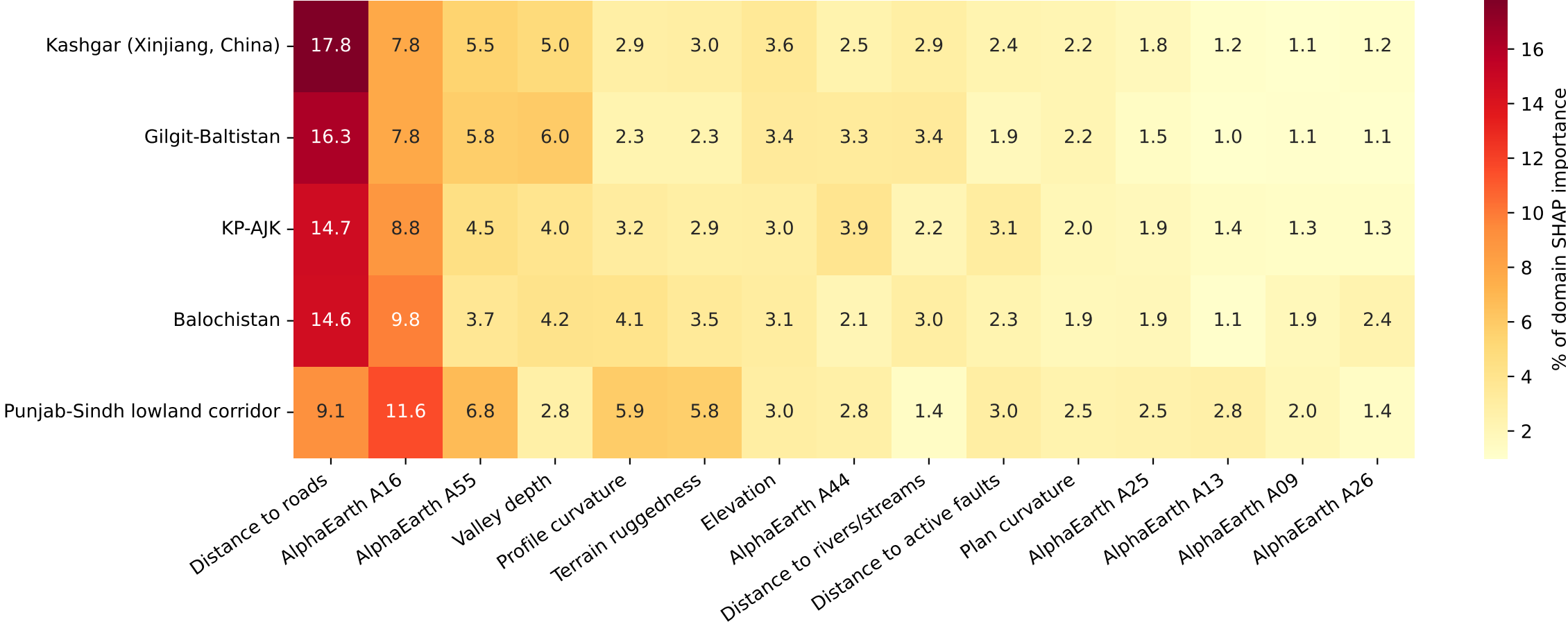
Domain-Specific Top Factors: Fused XGBoost TreeSHAP
