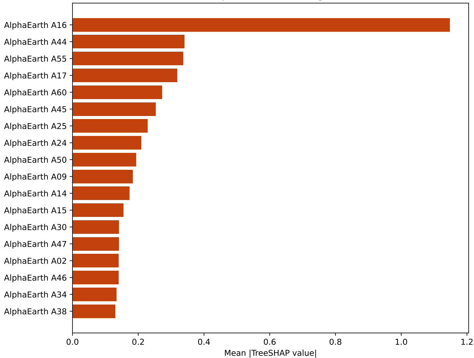
Domain TreeSHAP Importance: Balochistan AlphaEarth Embeddings
