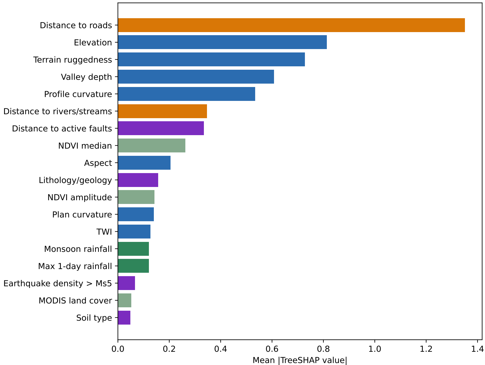
Domain TreeSHAP Importance: Balochistan Conventional
