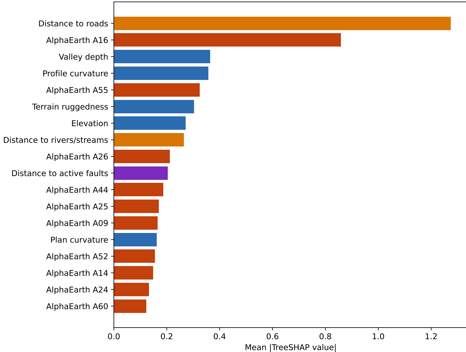
Domain TreeSHAP Importance: Balochistan Conventional + AlphaEarth Embeddings
