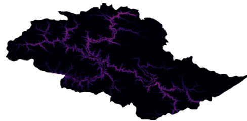
Reliability-aware score
