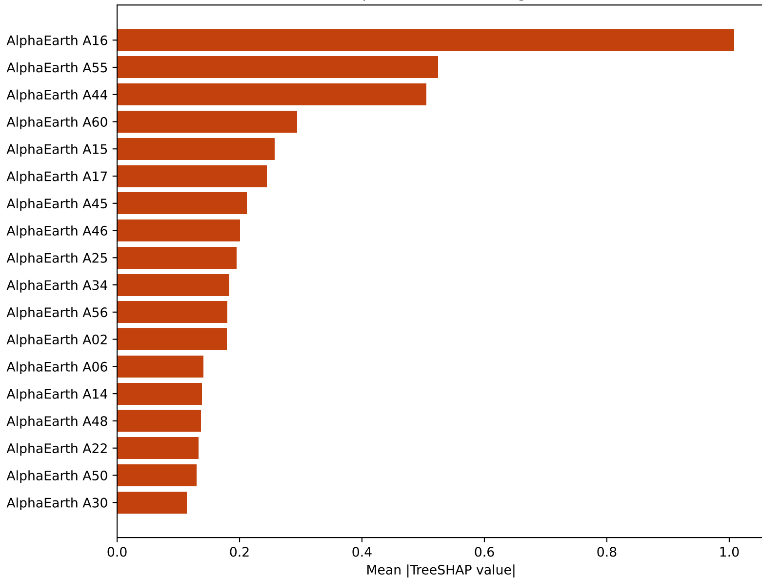
Domain TreeSHAP Importance: Gilgit-Baltistan AlphaEarth Embeddings
