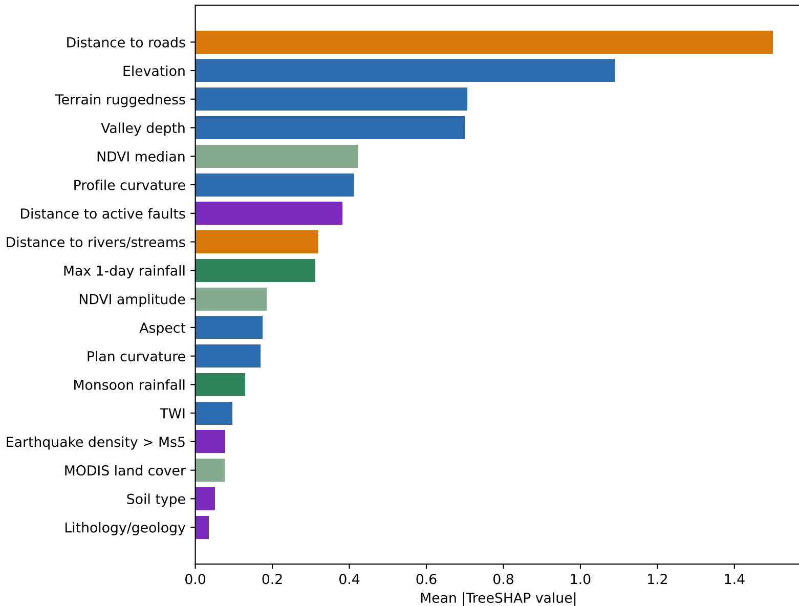
Domain TreeSHAP Importance: KP-AJK Conventional
