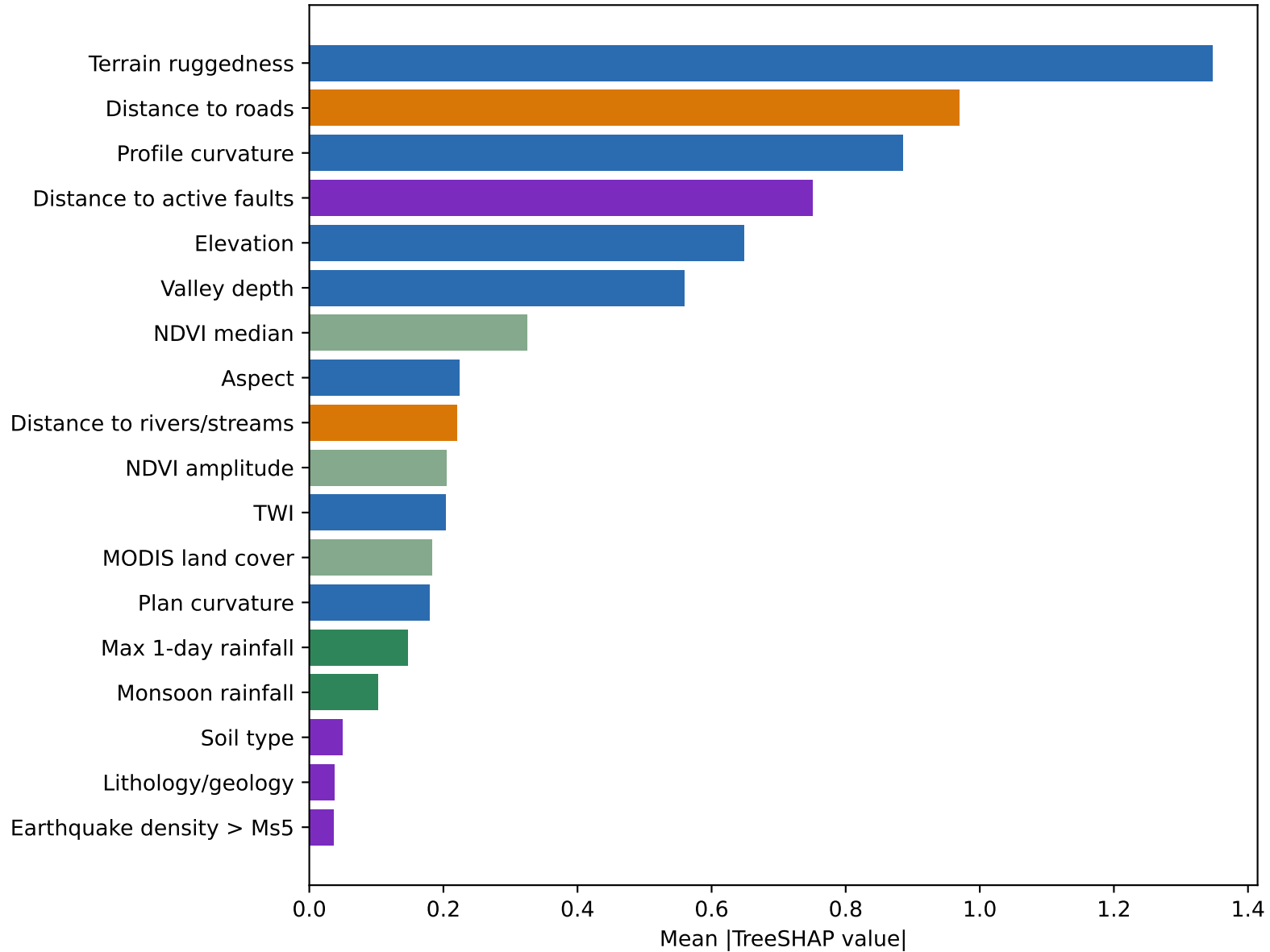
Domain TreeSHAP Importance: Punjab-Sindh lowland corridor Conventional
