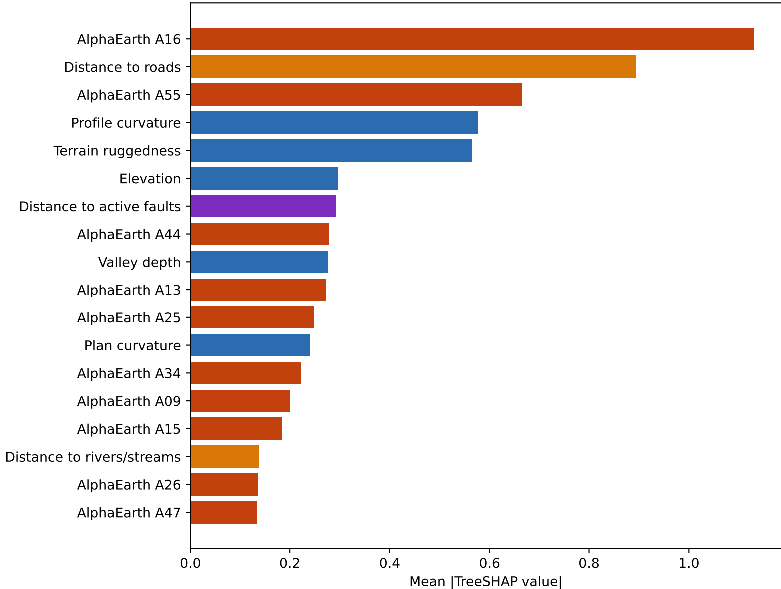
Domain TreeSHAP Importance: Punjab-Sindh lowland corridor Conventional + AlphaEarth Embeddings
