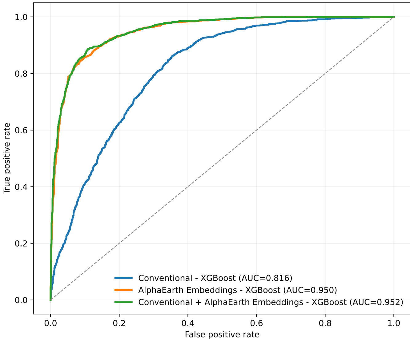
2018 Spatial-CV ROC Curves
