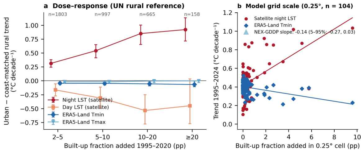
Figure 4. Dose–response of warming trends to urban growth. (a) Difference between trends in urbanising pixels and coast-matched rural pixels by class of added built-up fraction, for night-time and daytime LST and for ERA5-Land Tmin and Tmax sampled at the same pixels; rural land is defined by the UN Degree of Urbanisation. Error bars are 95% spatial block-bootstrap intervals; n is the number of urban pixels. (b) Night-time LST and ERA5-Land Tmin trends in the 104 NEX-GDDP-CMIP6 0.25^{\circ} cells over UAE land against the cell-mean added built-up fraction, with least-squares fits; the legend gives the corresponding NEX-GDDP-CMIP6 ensemble slope.
