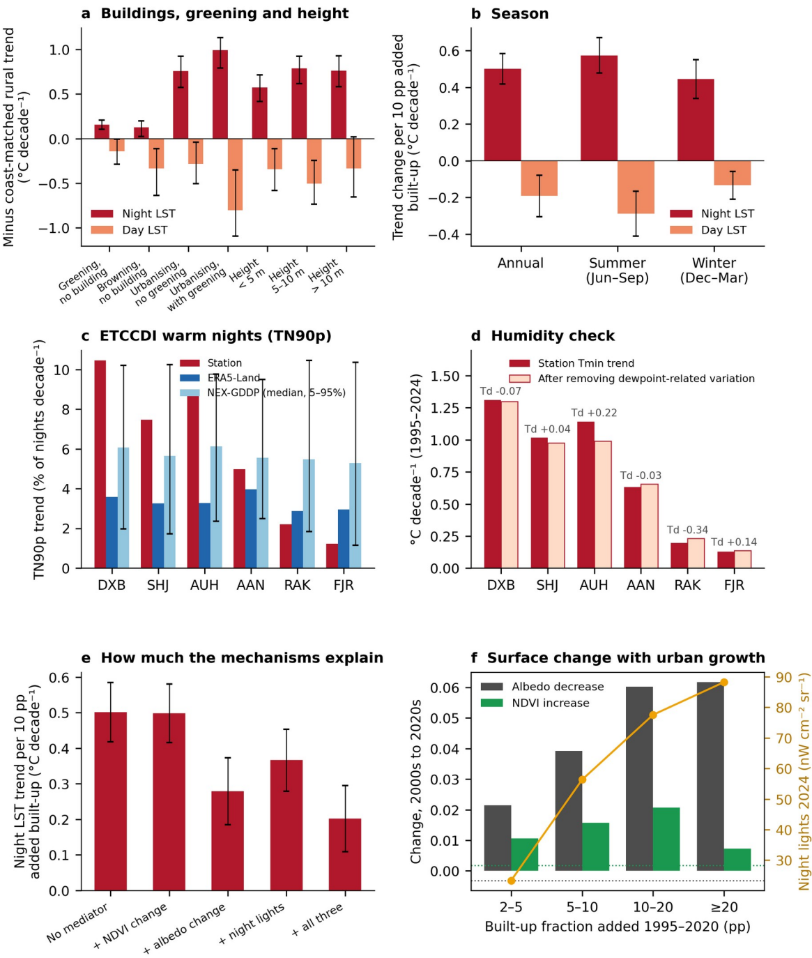
440 441 Figure 6. Mechanisms, alternative explanations and warm nights. (a) Night-time and daytime LST trend minus the 442 coast-matched rural trend for land that changed without building (greening, \Delta\text{NDVI} \geq 0.05 ; browning, \Delta\text{NDVI} \leq 443 -0.02 ), for urbanising land (added built-up fraction \geq 10 pp) without and with greening, and for urbanising pixels 444 ( \geq 5 pp) by mean building height ( < 5 m, 5–10 m, > 10 m). (b) Regression coefficient per 10 pp of added built-up 445 fraction for annual, summer and winter LST trends. (c) Trends in the ETCCDI warm-night index TN90p (base 446 period 1991–2020) at stations, the nearest ERA5-Land cell and NEX-GDDP-CMIP6 (median and 5–95% of 28 447 models). (d) Station Tmin trends before and after removing the component related to night-time dewpoint; labels 448 give the dewpoint trend ( ^{\circ}\text{C decade}^{-1} ). (e) The built-up coefficient for night-time LST when satellite-measured 449 mechanisms are added to the regression. (f) Decrease in albedo and change in NDVI between the early 2000s and
