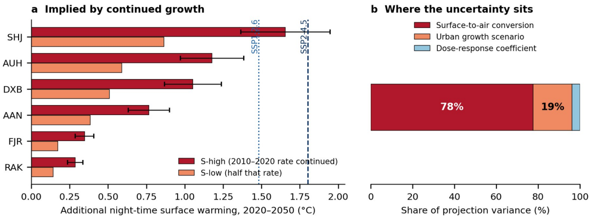
556 Figure 7. The urban warming increment to 2050 and where its uncertainty lies. (a) Additional night- 557 time surface warming between 2020 and 2050 within 5 km of each station, under continuation of the 558 observed 2010–2020 built-up growth rate (S-high) and half that rate (S-low); error bars are 95% 559 confidence intervals from the dose–response. Vertical lines give the NEX-GDDP-CMIP6 UAE-area 560 Tmin change for 2041–2060 relative to 1995–2014 under two scenarios; those are 2 m air 561 temperatures and the bars are surface temperatures, so the comparison shows relative magnitude 562 rather than a common variable. (b) Share of the projection variance contributed by the surface-to-air 563 conversion, the built-up growth scenario and the dose–response coefficient. Station codes as in Fig. 564 1.
