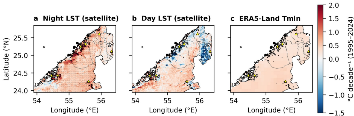
Figure 3. Theil–Sen trends for 1995–2024 over the northern UAE. (a) Night-time and (b) daytime satellite land-surface temperature (LST), with stippling where the Benjamini–Hochberg false-discovery rate is below 5%. (c) ERA5-Land Tmin on the same grid. Black contours enclose areas where built-up fraction increased by at least 10 percentage points between 1995 and 2020; triangles mark stations.
