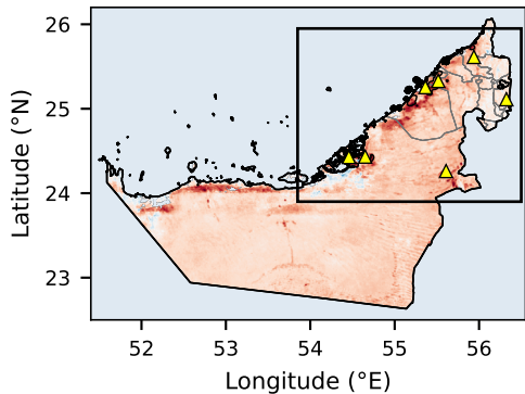
d Night-time LST, whole UAE
