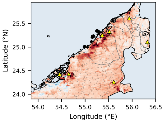
a Night-time LST
