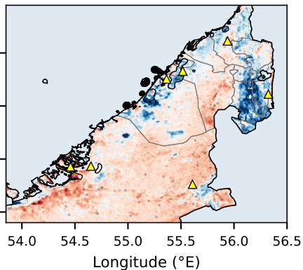
b Day-time LST
