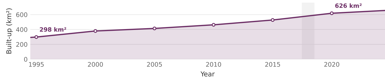
c UAE built-up surface · GHS-BUILT-S
