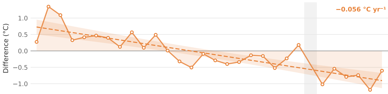
b Day-time LST · urbanising – rural
