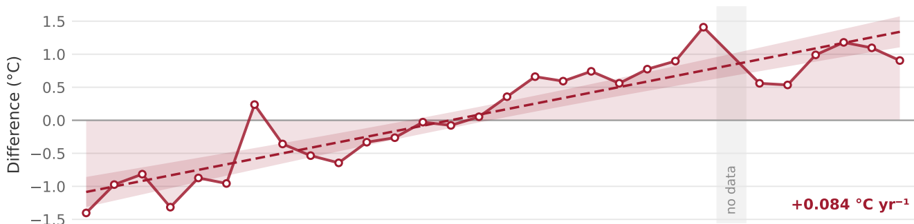
a Night-time LST · urbanising – rural
