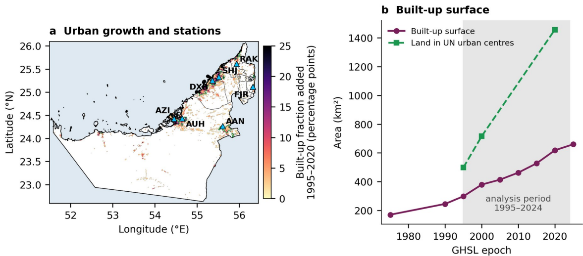
Figure 1. Urban growth and station network. (a) Increase in built-up fraction between 1995 and 2020 from GHS-BUILT-S (percentage points, shown where at least 1 pp); grey shading marks areas already at least 5% built up in 1995 and green outlines mark UN urban centres in 2020. Triangles show the HadISD stations: DXB, Dubai International; SHJ, Sharjah; AUH, Abu Dhabi International; AZI, Al Bateen; AAN, Al Ain; RAK, Ras Al Khaimah; FJR, Fujairah. (b) UAE built-up surface by GHSL epoch, and land in UN urban centres, for which the settlement grid is available for 1995, 2000 and 2020 only; shading marks the 1995–2024 analysis period.
