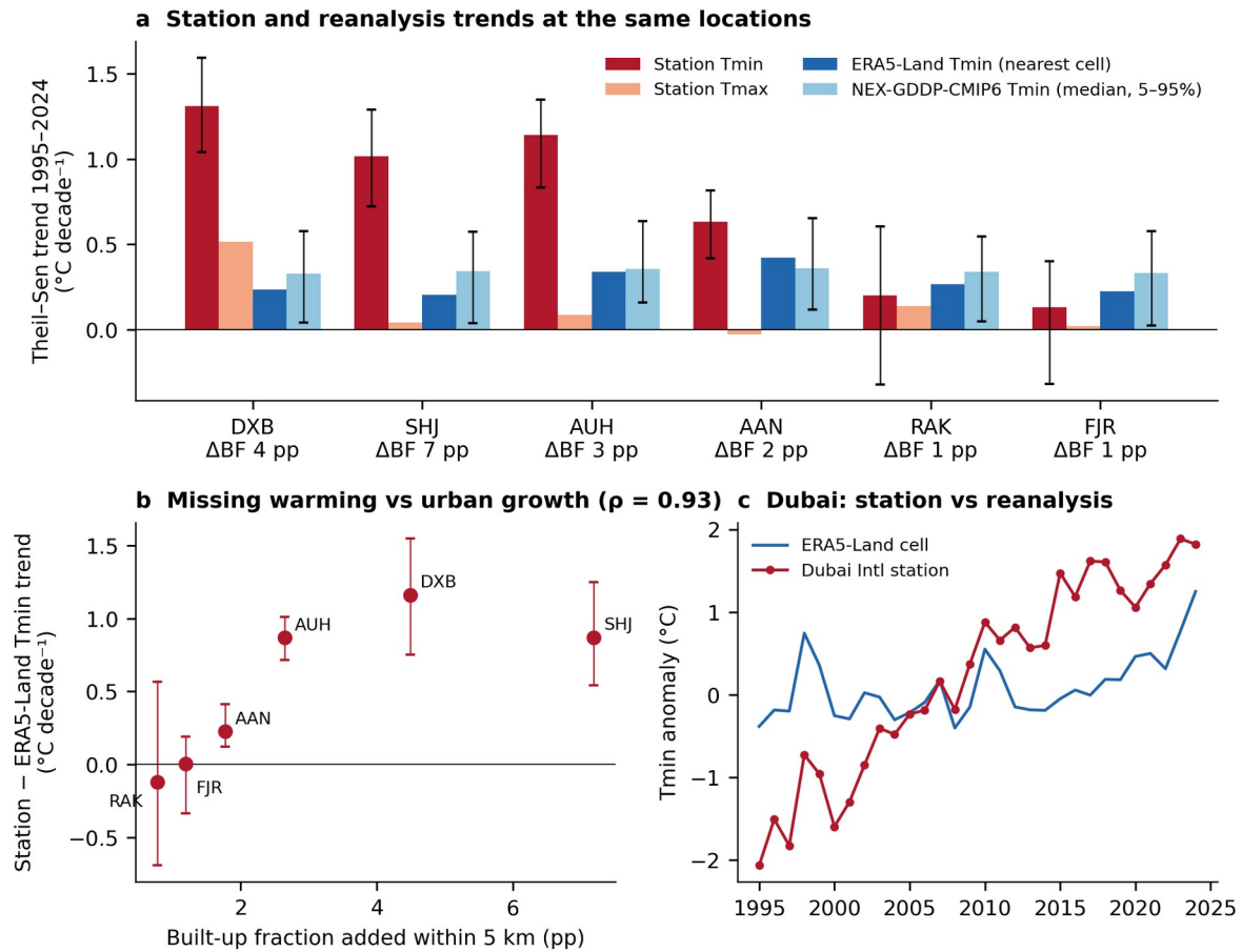
298 299 Figure 2. Station night-time warming and the regional products. (a) Theil–Sen trends for 1995–2024 300 in station Tmin (with 95% moving-block-bootstrap intervals) and Tmax, ERA5-Land Tmin at the 301 nearest cell, and NEX-GDDP-CMIP6 Tmin (median and 5–95% range of 28 models) at the same 302 locations; labels give the built-up fraction added within 5 km between 1995 and 2020 ( \Delta BF). (b) 303 Station-minus-ERA5-Land Tmin trend (urban warming increment) against \Delta BF within 5 km, with 304 95% intervals. (c) Annual Tmin anomalies at Dubai International and the nearest ERA5-Land cell, 305 relative to 1995–2020.
