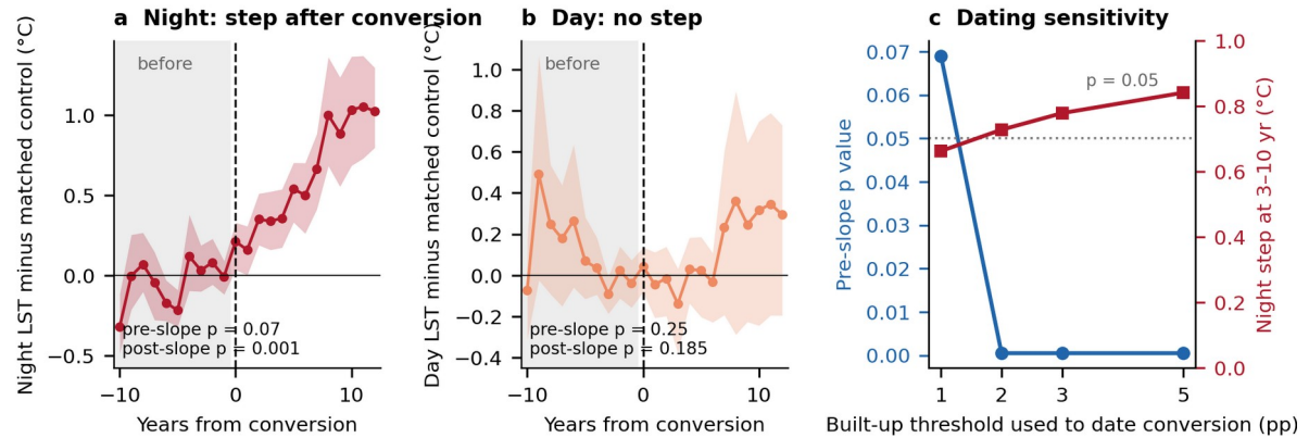
Figure 5. Night-time land-surface temperature before and after built-up conversion. Each treated pixel is differenced against the mean of never-built control pixels in the same coastal-distance band and emirate, and normalised to its own mean over the five years before conversion; shading is the 95% block-bootstrap interval over 0.25^{\circ} blocks. (a) Night-time and (b) day-time difference from matched controls against years from conversion, for the treated pixels of the 2005, 2010 and 2015 cohorts (432 at night, 433 by day); the dashed line marks the conversion date and grey shading the pre-conversion window. (c) Sensitivity to the built-up threshold used to date conversion: the bootstrap p value of the pre-conversion slope (left axis) and the mean night-time level three to ten years after conversion (right axis). The estimated effect is stable across datings; only the timing test depends on the choice. Slopes, levels and their p values are estimated inside each bootstrap replicate.
