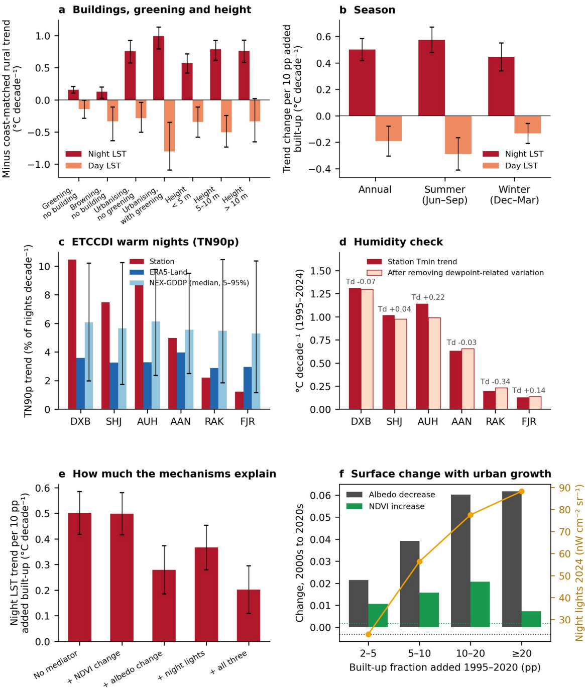
438 439 Figure 6. Mechanisms, alternative explanations and warm nights. (a) Night-time and daytime LST trend minus the 440 coast-matched rural trend for land that changed without building (greening, \Delta\text{NDVI} \geq 0.05 ; browning, \Delta\text{NDVI} \leq 441 -0.02 ), for urbanising land (added built-up fraction \geq 10 pp) without and with greening, and for urbanising pixels 442 ( \geq 5 pp) by mean building height ( < 5 m, 5–10 m, > 10 m). (b) Regression coefficient per 10 pp of added built-up 443 fraction for annual, summer and winter LST trends. (c) Trends in the ETCCDI warm-night index TN90p (base 444 period 1991–2020) at stations, the nearest ERA5-Land cell and NEX-GDDP-CMIP6 (median and 5–95% of 28 445 models). (d) Station Tmin trends before and after removing the component related to night-time dewpoint; labels 446 give the dewpoint trend ( ^{\circ}\text{C decade}^{-1} ). (e) The built-up coefficient for night-time LST when satellite-measured 447 mechanisms are added to the regression. (f) Decrease in albedo and change in NDVI between the early 2000s and
