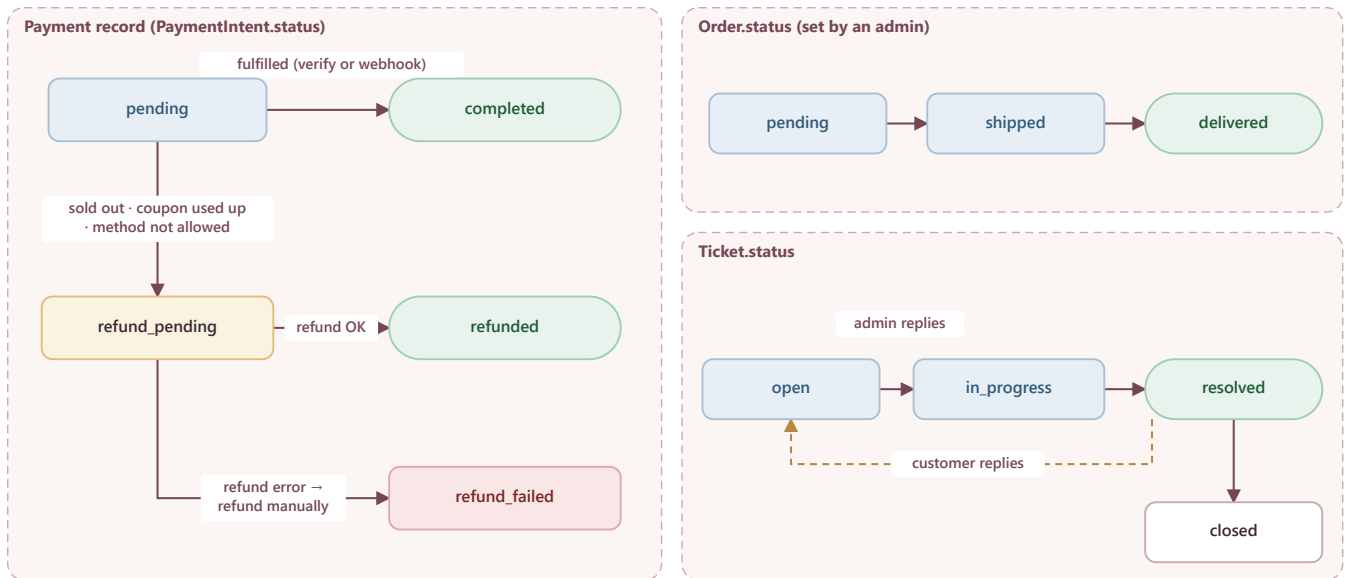
Figure 6.5 — Status lifecycles for payment records, orders and tickets
