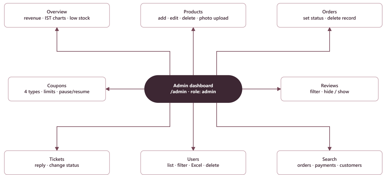
Figure 4.6 — The admin dashboard and its tabs
