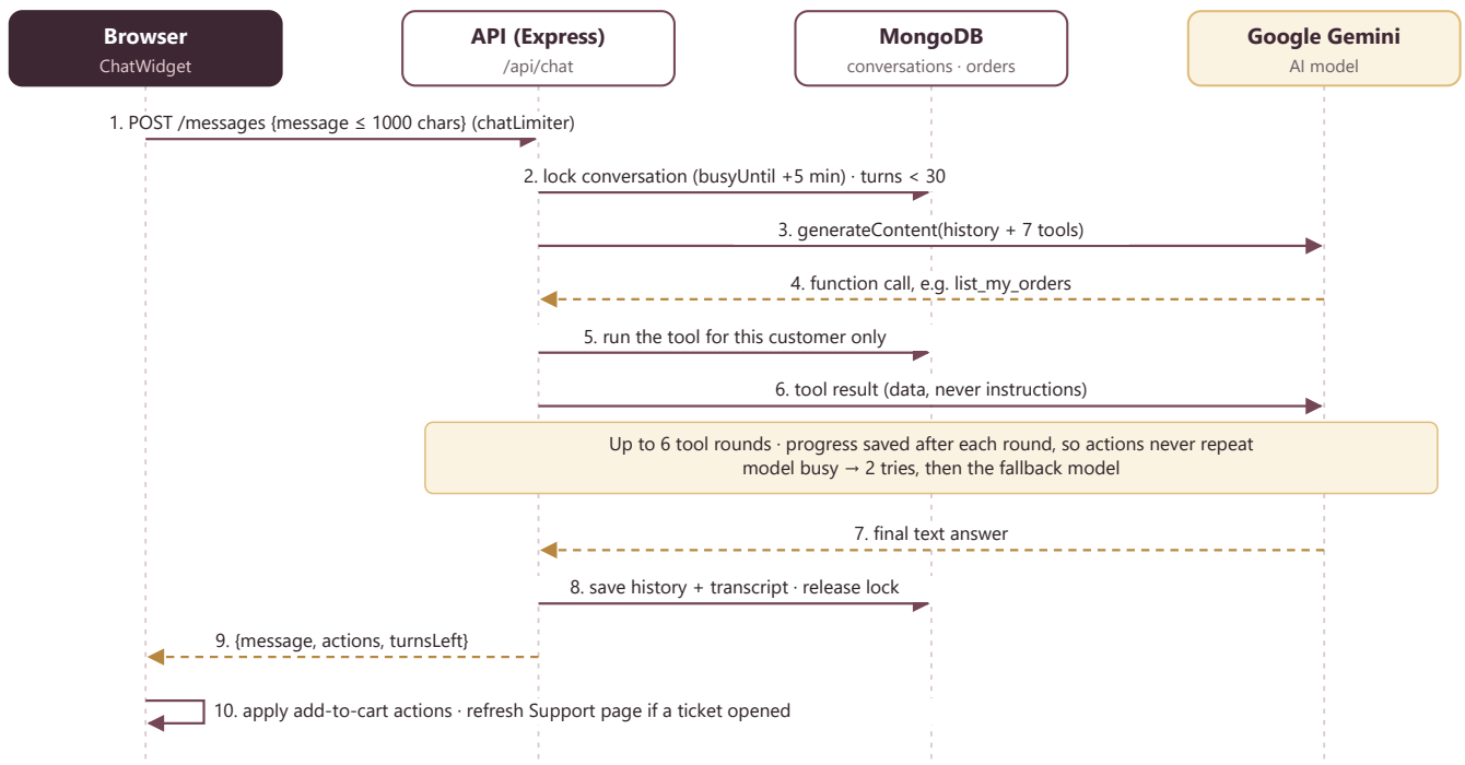
Figure 5.6 — POST /api/chat/messages and the tool loop
