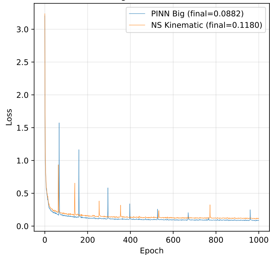
Training Loss (linear scale)
