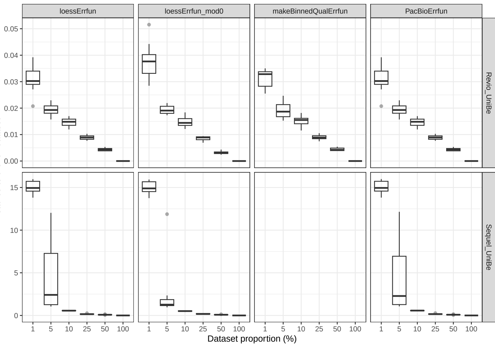
Distance to the full dataset
