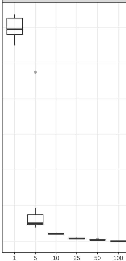
loessErrfun_mod0
