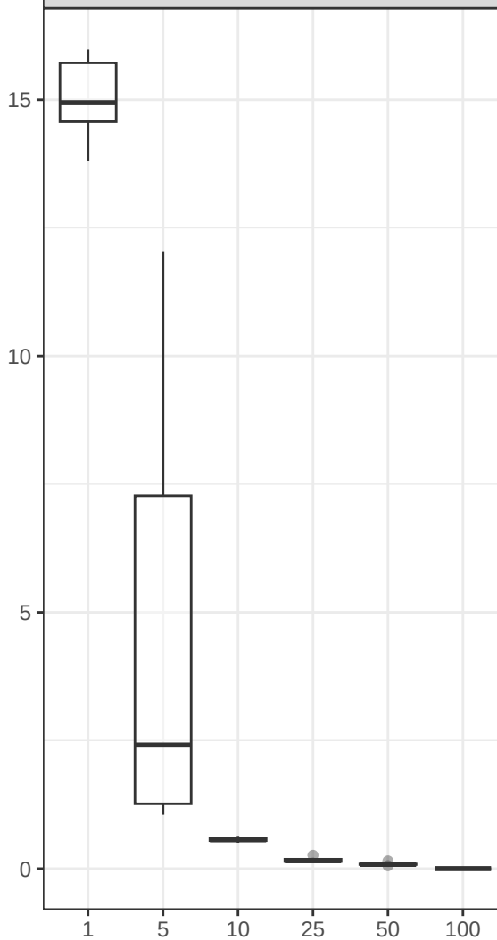
loessErrfun
