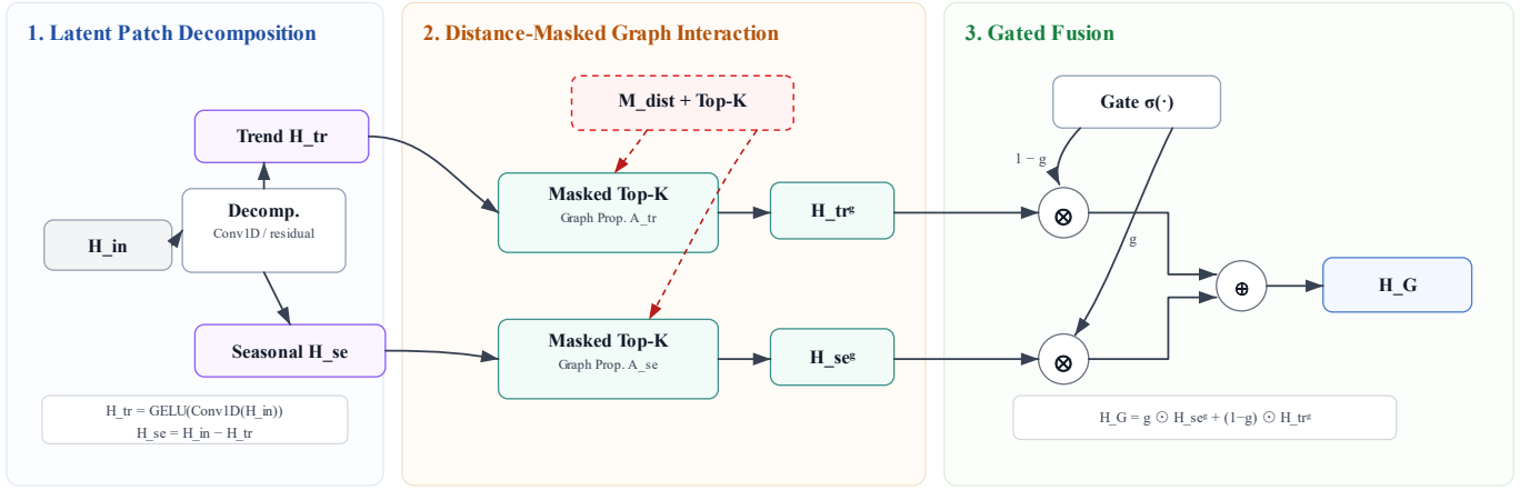
Fig. 3. Detailed architecture of R-STM. The latent representation is decomposed into trend and seasonal manifolds. Each branch performs distance-masked Top- K graph propagation with branch-specific routing, and the resulting graph-enhanced manifolds are fused through a learnable gate.
