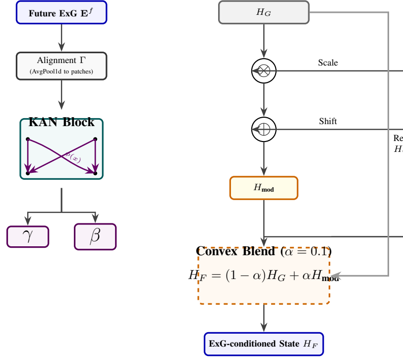
Fig. 4. Mechanics of K-AMC. Future exogenous drivers are aligned and processed through a KAN block (featuring learnable spline edge functions) to produce dynamic scale and shift parameters. The final conditioned state is derived via a stable convex blending mechanism.
