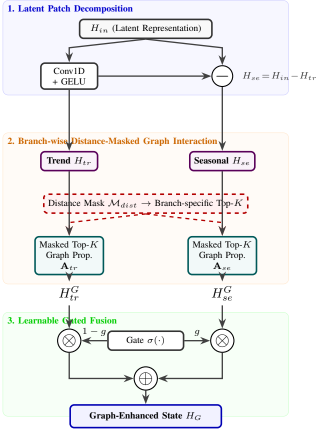
Fig. 3. Detailed architecture of R-STMF. The input latent representation H_{in} undergoes manifold decomposition. The seasonal (residual) and trend (Conv1D) components independently undergo branch-wise distance-masked graph propagation prior to gated fusion.
