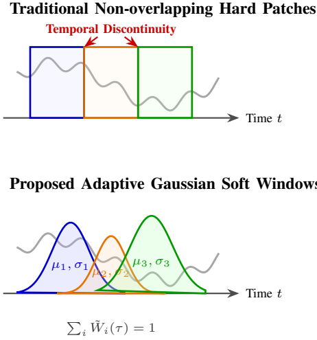
Fig. 2. Mechanics of AGSP. By replacing discrete sequence chunking with continuous, differentiable density windows, the model autonomously mitigates boundary artifacts and preserves temporal continuity. Each soft window is parameterized by a learnable center \mu_i and bandwidth \sigma_i , with overlapping weights dynamically normalized.
