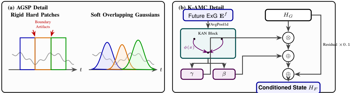
Fig. 2. Internal mechanics of the coupled modules. (a) AGSP replaces discrete sequence chunking with continuous, differentiable density windows, reducing boundary artifacts. (b) K-AMC leverages Kolmogorov-Arnold Networks (KAN) to map future exogenous features into dynamic scale ($\gamma$) and shift ($\beta$) parameters for conditional modulation.
