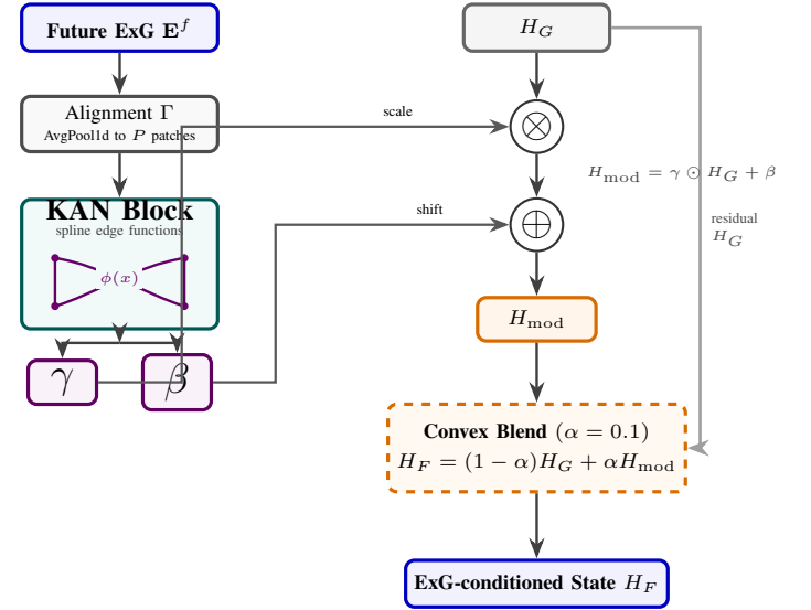
Fig. 4. Mechanics of K-AMC. Future exogenous drivers are aligned to the patch scale and processed through a KAN block with learnable spline edge functions to produce dynamic scale and shift parameters. The modulated state is combined with the original graph-enhanced state through a stable convex blending mechanism.
