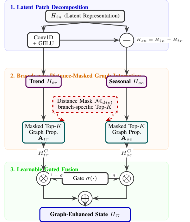
Fig. 3. Detailed architecture of R-STMF. The input latent representation H_{in} is decomposed into trend and seasonal manifolds. The two branches independently perform distance-masked Top-K graph propagation and are then recombined through learnable gated fusion.
