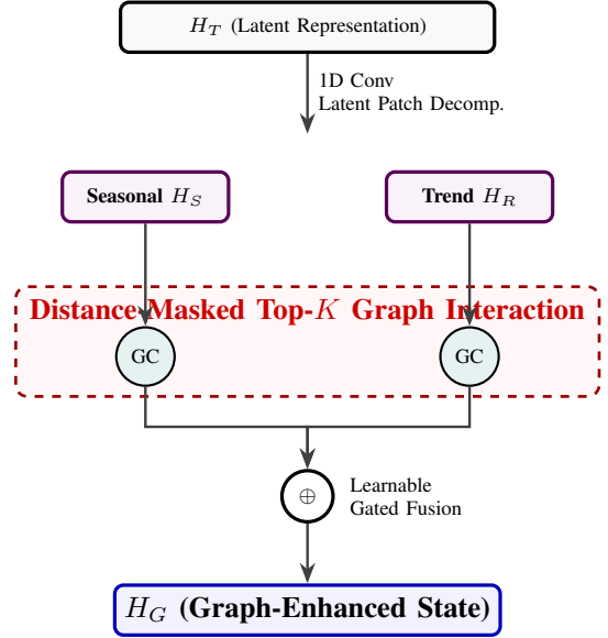
Fig. 3. Detailed architecture of R-STMf. Latent patch sequences are decomposed into seasonal and trend manifolds, which independently undergo distance-masked graph convolution prior to gated fusion.
