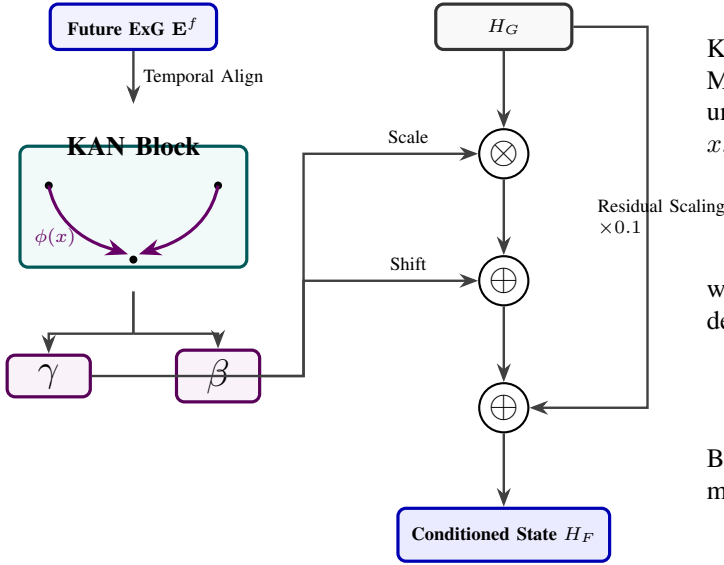
Fig. 4. Mechanics of K-AMC. Future exogenous drivers are aligned and processed through a KAN block to produce dynamic scale and shift parameters, which then non-linearly modulate the graph-enhanced latent state.
