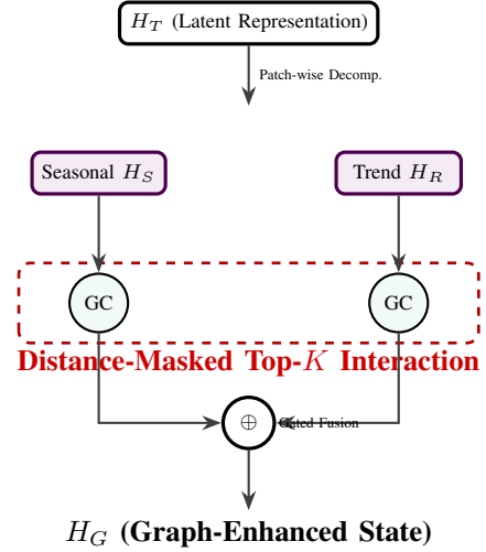
Fig. 3. Detailed architecture of R-STMF. Latent patch sequences are decomposed into seasonal and trend manifolds, which independently undergo distance-masked graph convolution prior to gated fusion.
