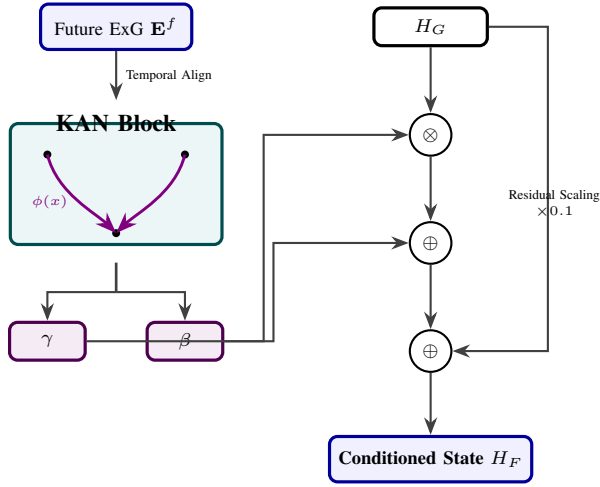
Fig. 4. Mechanics of K-AMC. Future exogenous drivers are aligned and processed through a KAN block to produce dynamic scale and shift parameters, which then non-linearly modulate the graph-enhanced latent state.
