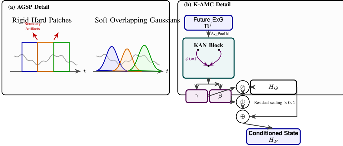
Fig. 2. Internal mechanics of the coupled modules. (a) AGSP replaces discrete sequence chunking with continuous, differentiable density windows, reducing boundary artifacts. (b) K-AMC leverages Kolmogorov-Arnold Networks (KAN) to map future exogenous features into dynamic scale ( \gamma ) and shift ( \beta ) parameters for conditional modulation.
