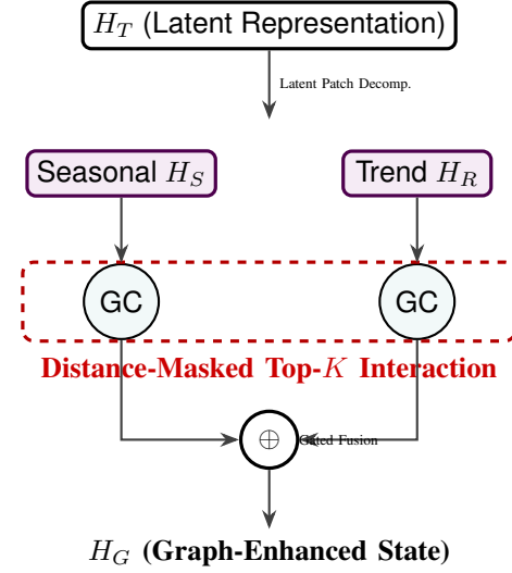
Fig. 3. Detailed architecture of R-STMF. Latent patch sequences are decomposed into seasonal and trend manifolds, which independently undergo distance-masked graph convolution prior to gated fusion.
