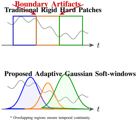
Fig. 2. Mechanics of AGSP. By replacing discrete sequence chunking with continuous, differentiable density windows, the model autonomously mitigates boundary artifacts and atmospheric noise.
