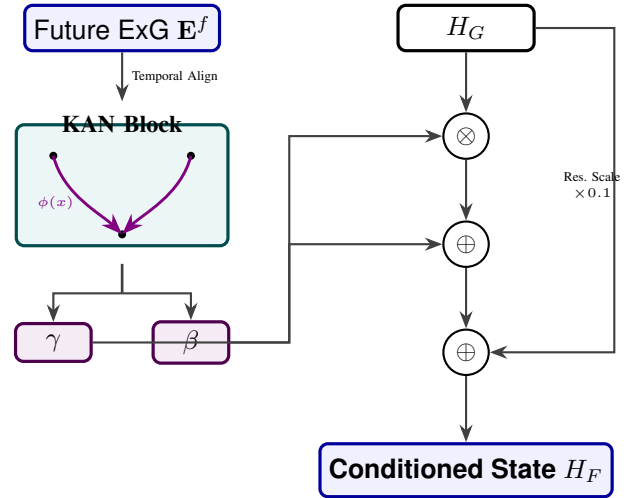
Fig. 4. Mechanics of K-AMC. Future exogenous drivers are aligned and processed through spline-based KAN edges to produce dynamic modulation parameters.
