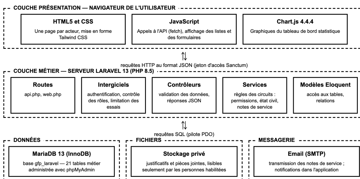
Figure 4 : Architecture technique de la plateforme
