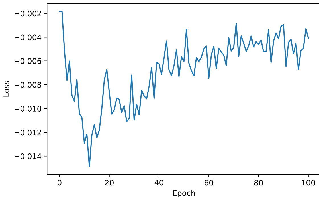
Actor Loss
