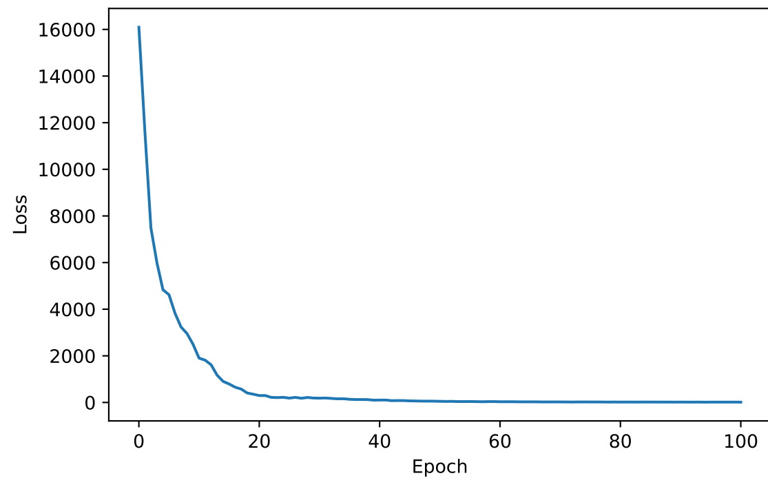
Critic Loss
