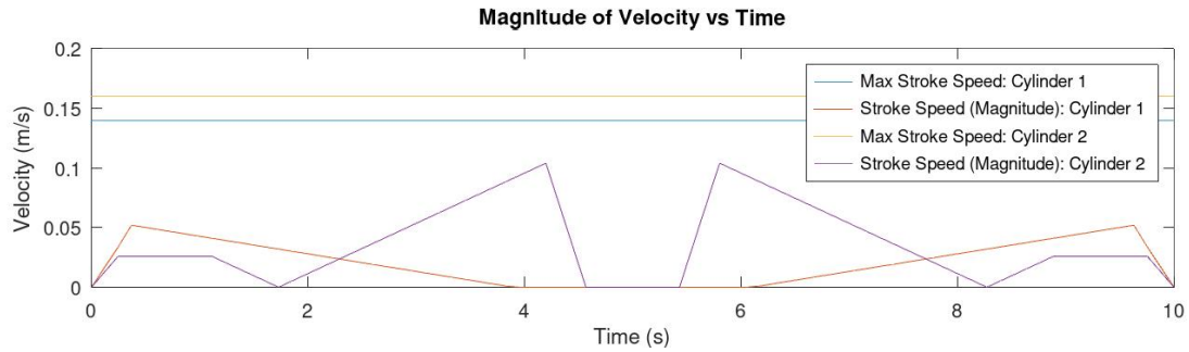
Figure 4: Determination of being under the maximum stroke velocity throughout cycle
